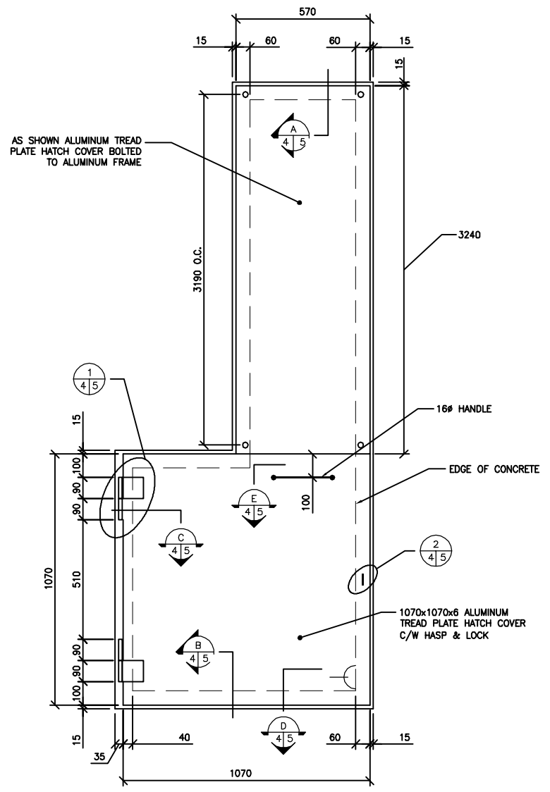
3 DETAIL 1:10
