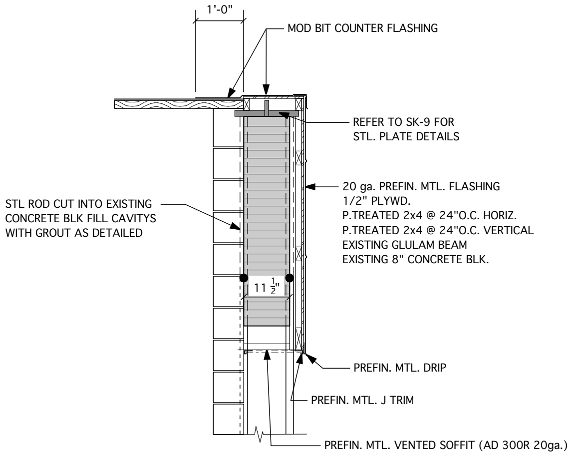
1 SECTION DETAIL SK-13 SCALE: 1/2" = 1'-0"
