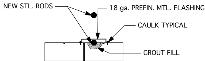
2 SECTION DETAIL SK-13 SCALE: 1/2" = 1'-0"
