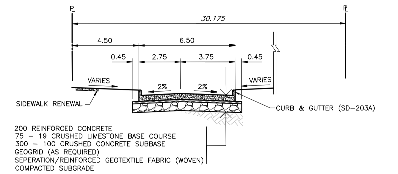
1 BURROWS AVENUE CROSS SECTION HOR 1:150, VER 1:75
