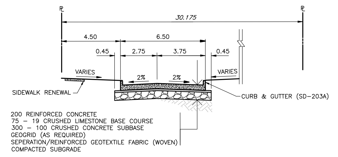
1 BURROWS AVENUE CROSS SECTION HOR 1:150, VER 1:75
