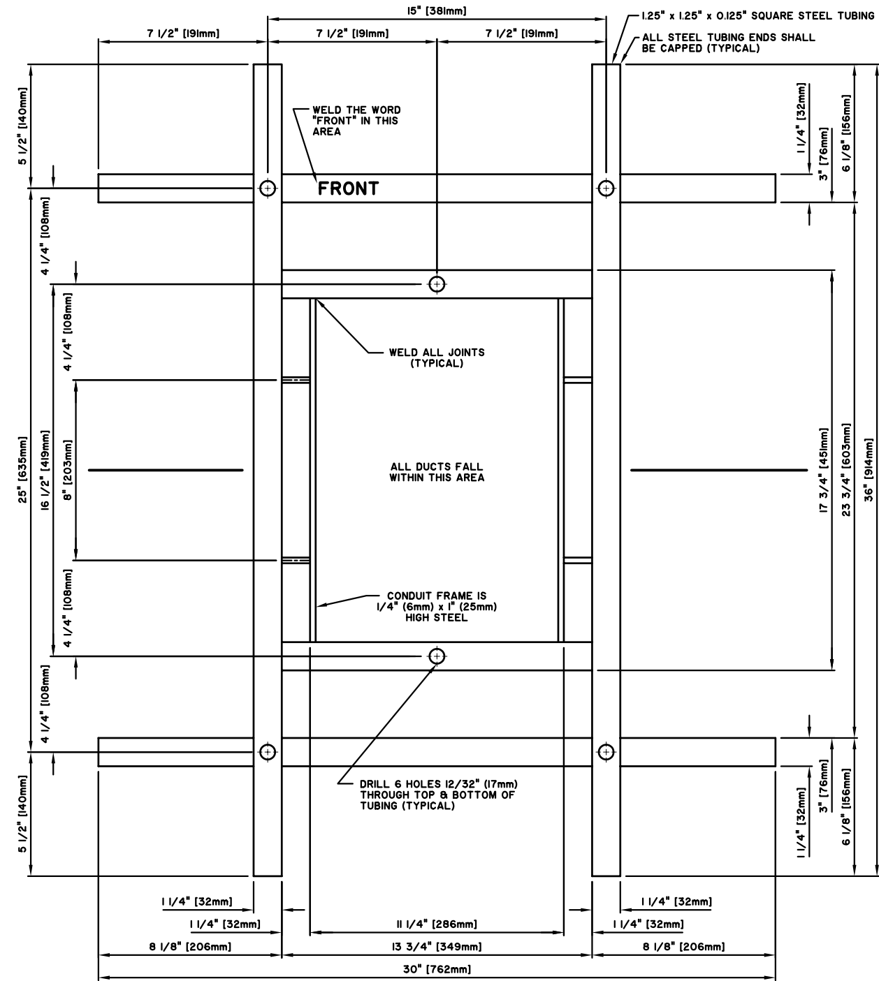
PLAN VIEW SCALE 3" = 1'-0"
