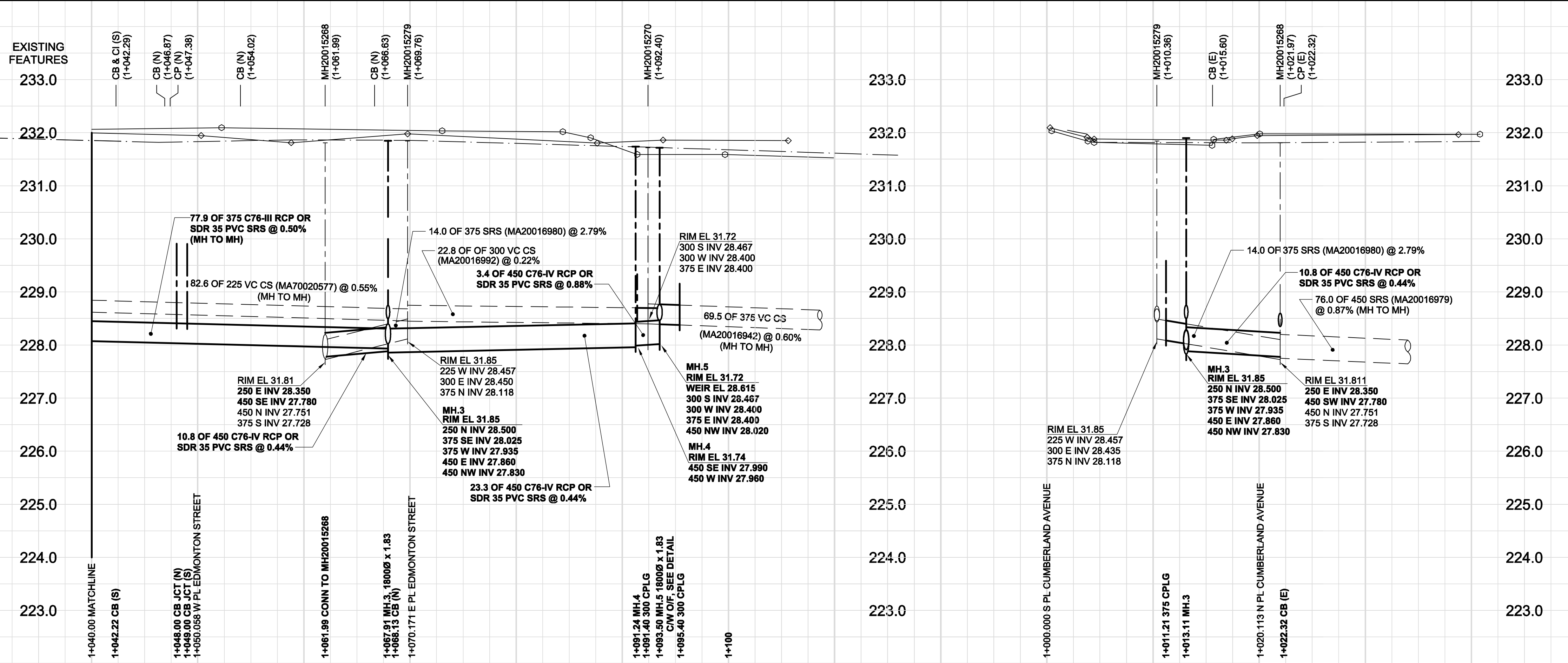
SECTION B SCALE 1:250 CHAINAGE ALONG E PL EDMONTON STREET
