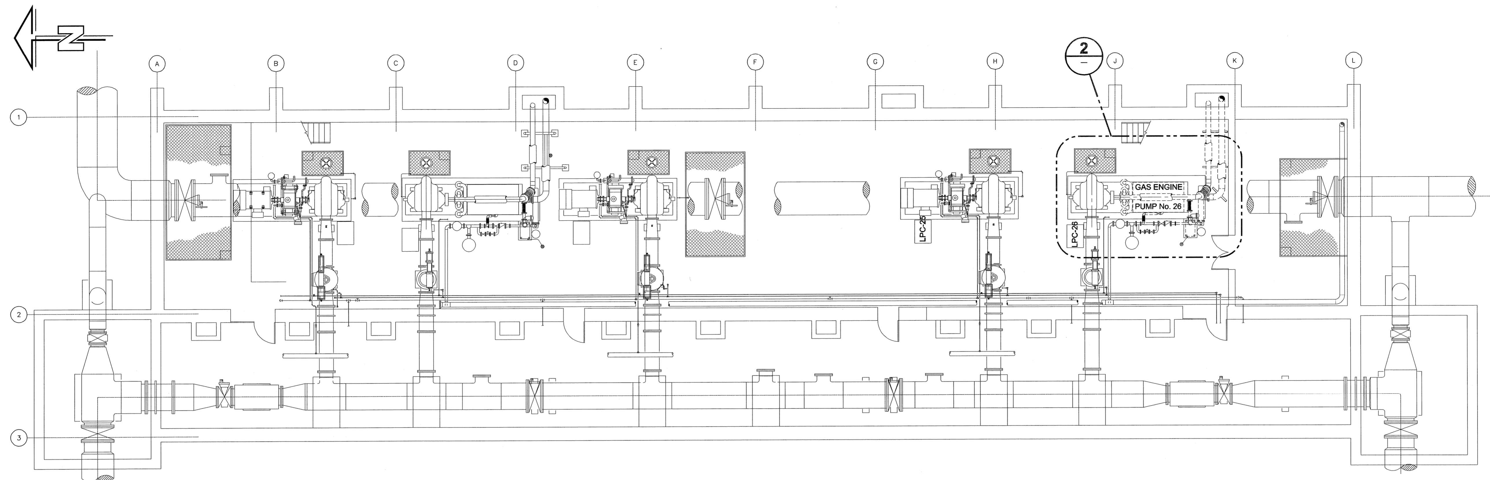
PLAN 1 0 1000 2000 3000 mm SCALE 1:100
