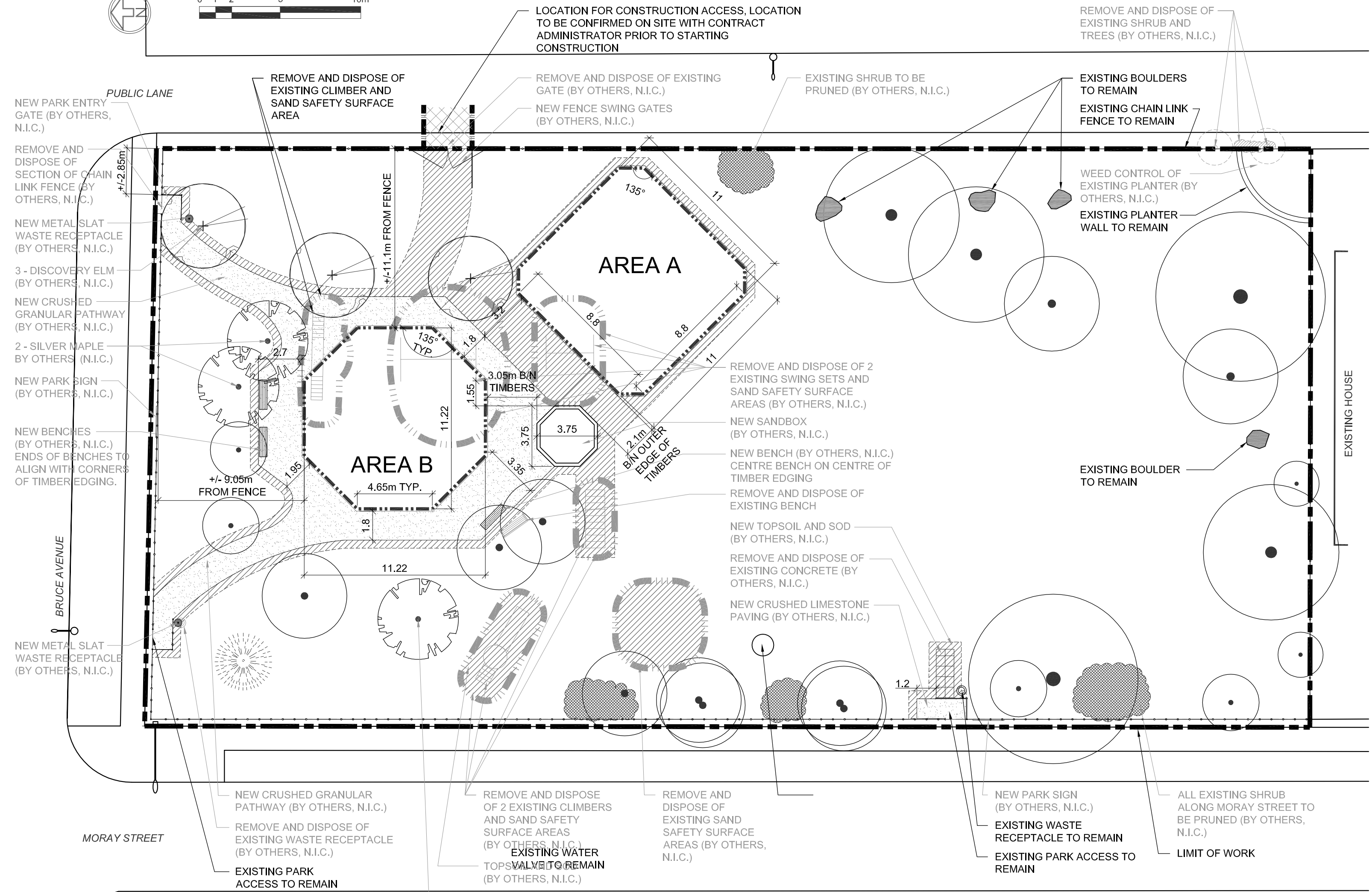
1 MORAY & BRUCE PLAYGROUND - PROPOSED SITEPLAN SCALE 1:200
