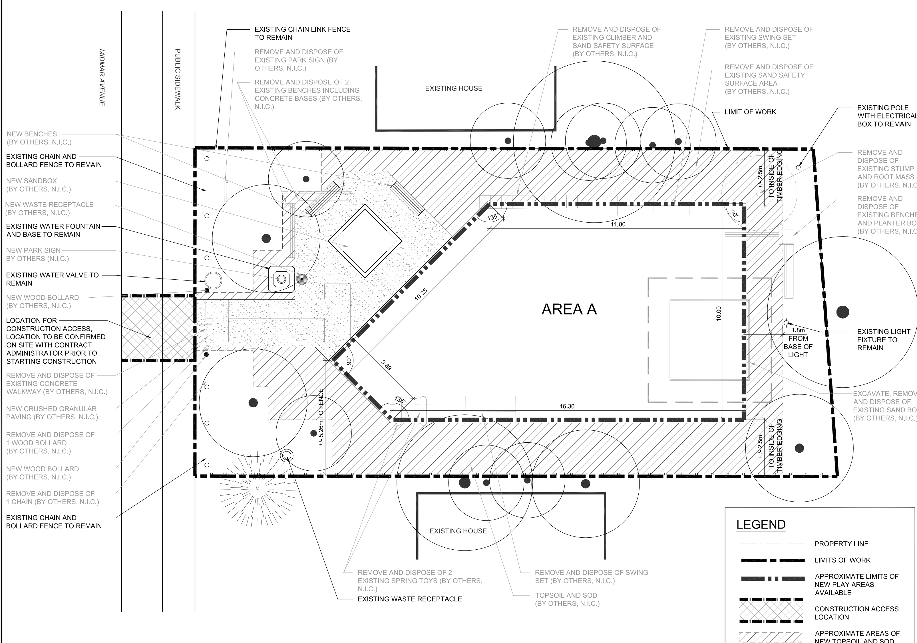
1 GALMAR PARK - PROPOSED SITEPLAN PE-GP1 SCALE 1:100
