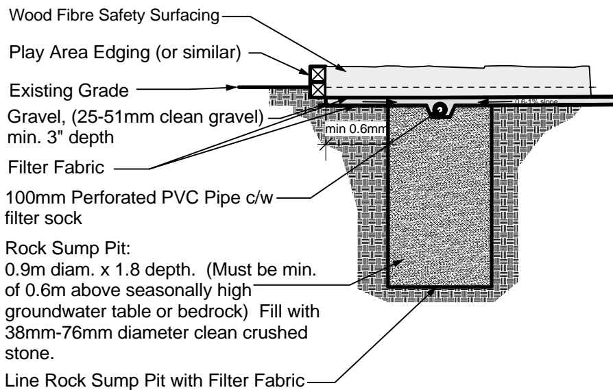
Section NTS
