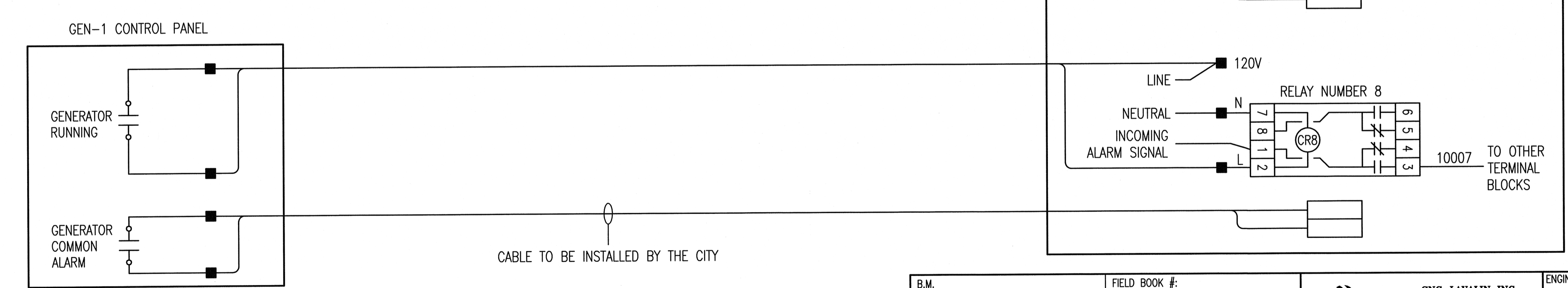
WIRING DIAGRAM - MCC-1 CONTROL - GENERATOR CONTROL PANEL NTS
