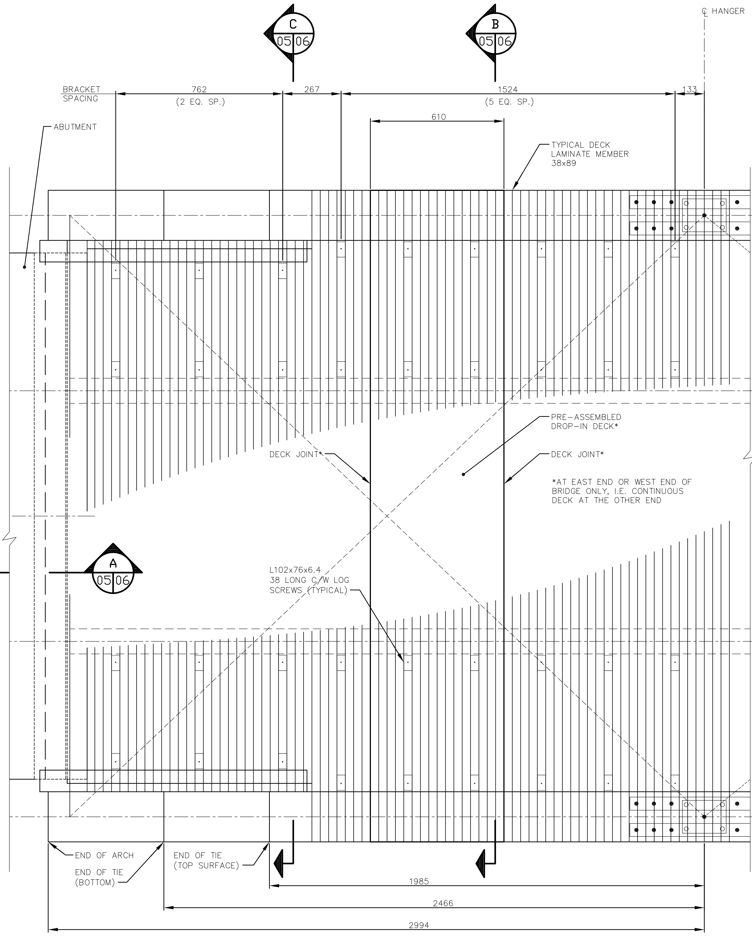
DECK REPLACEMENT AT BRIDGE ENDS SCALE: 1:10
