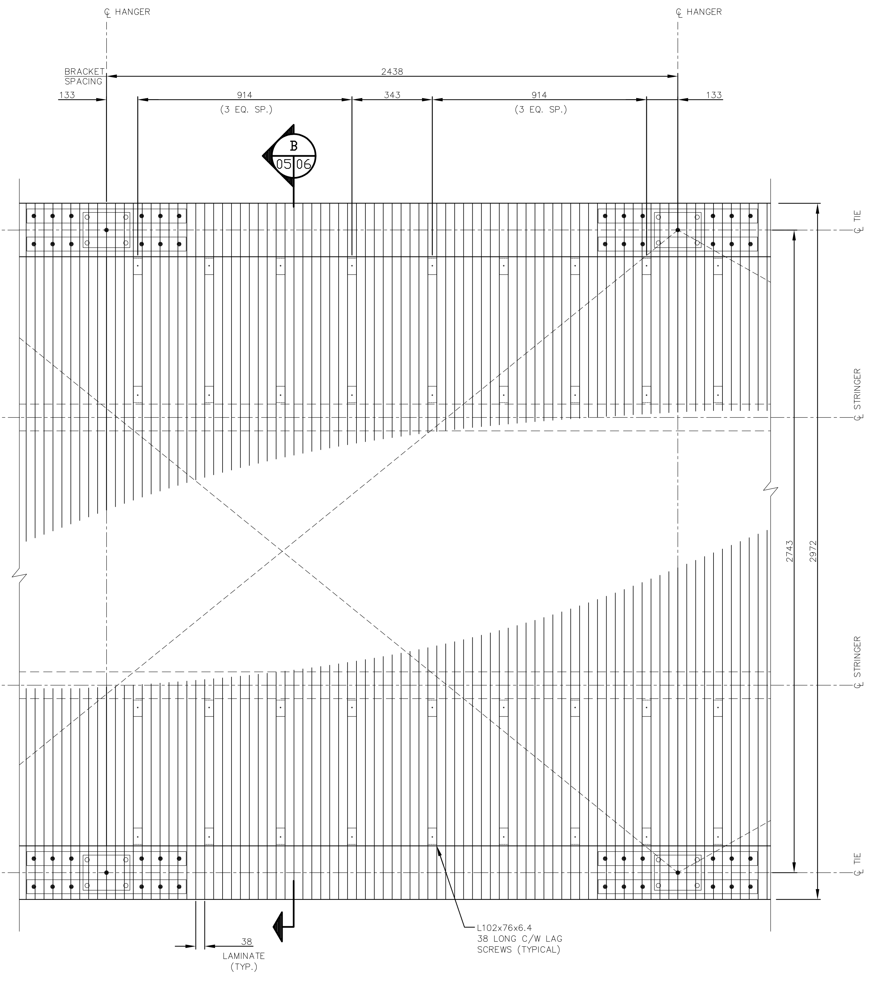
DECK REPLACEMENT (TYPICAL PANEL) SCALE: 1:10
