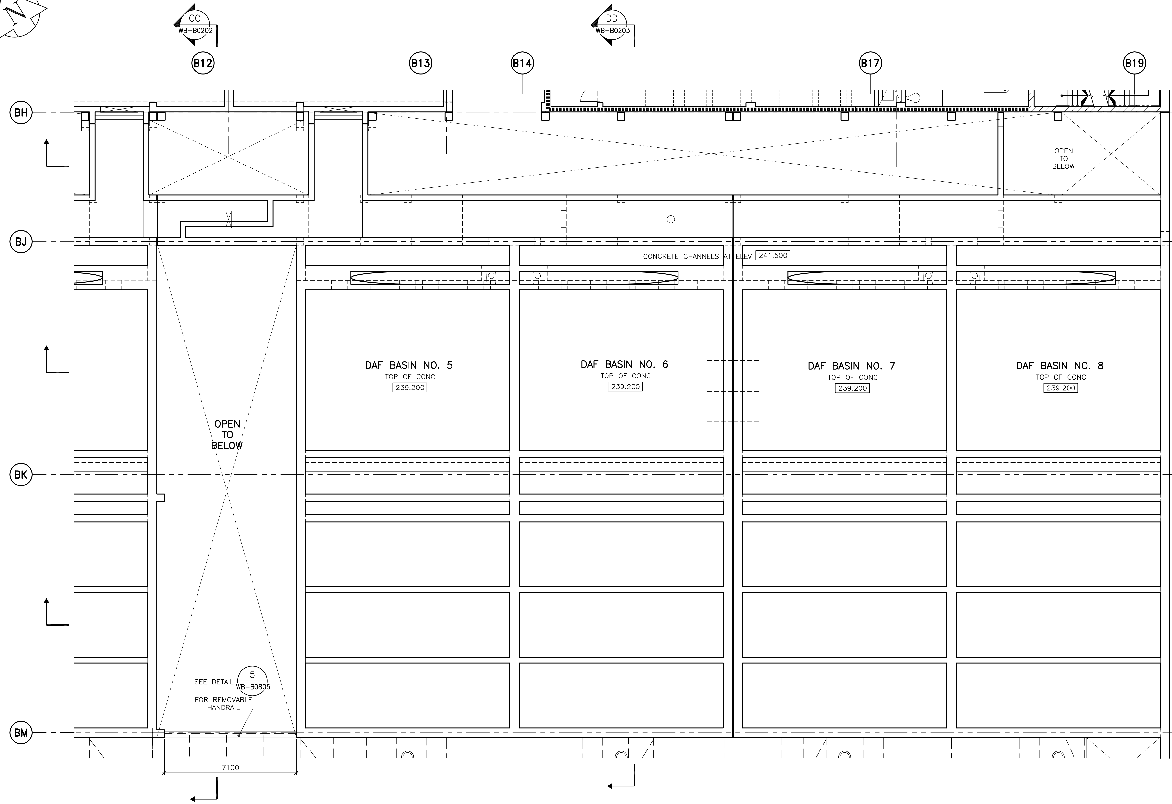
1 PARTIAL PLAN - DAF TANKS AND CHANNEL AREA (SECOND FLOOR) WB-B0127 1:100
