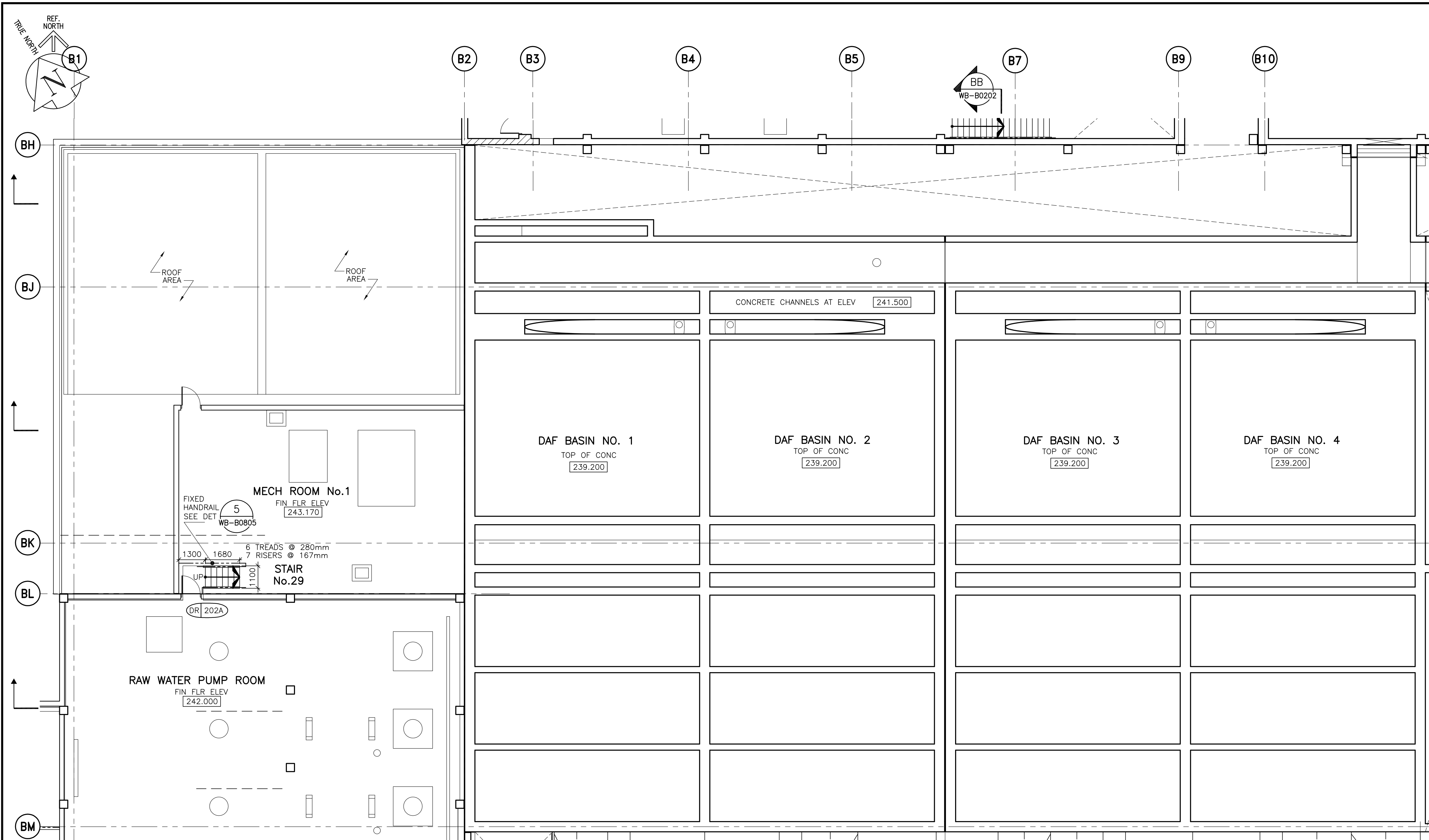
1 PARTIAL PLAN - DAF TANK & MECHANICAL RM NO. 1 AREA (SECOND FLOOR) WB-B0126 1:100
