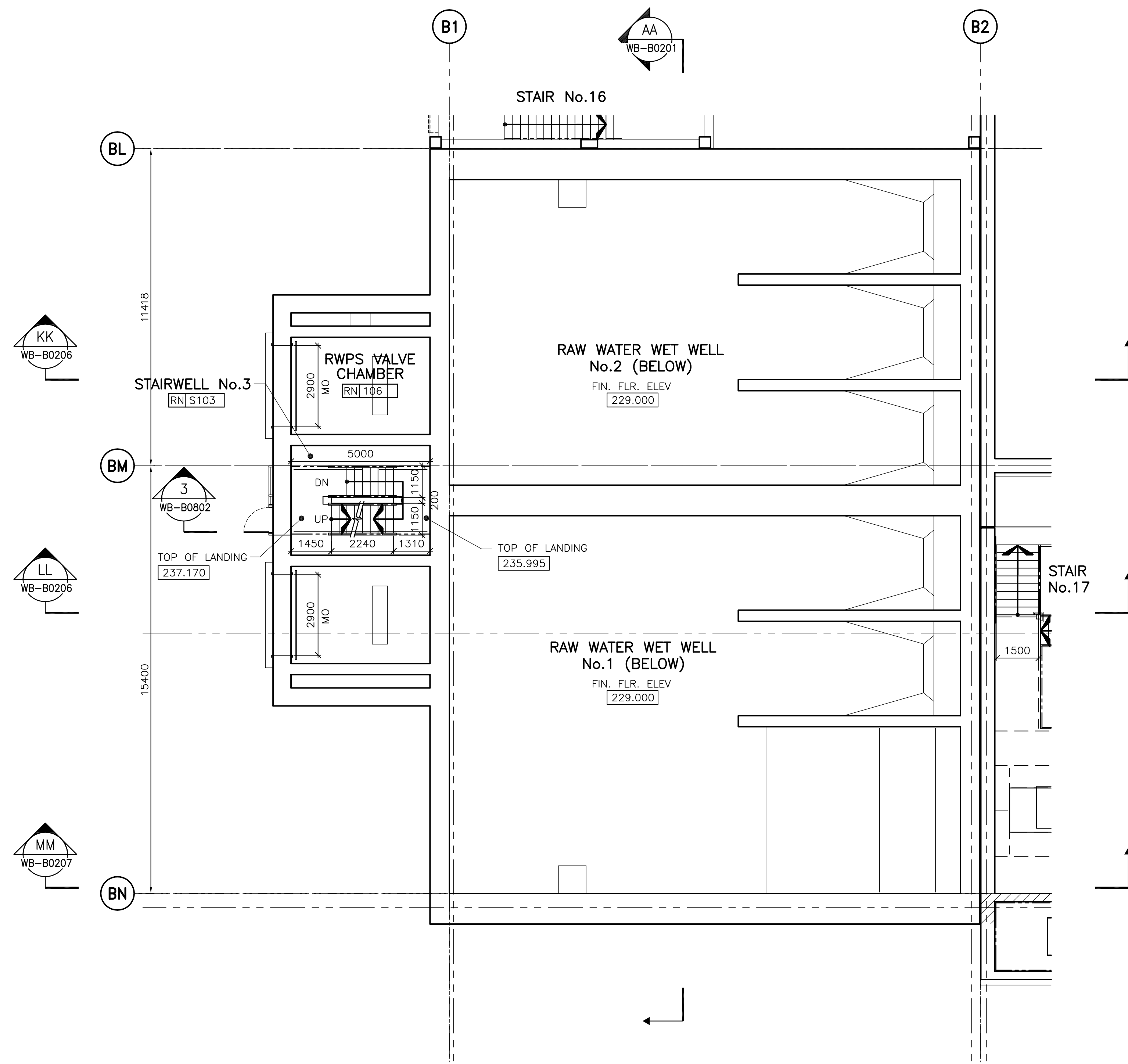
1 PARTIAL PLAN - RAW WATER PUMP STATION (FIRST FLOOR) WB-B0118 1:100
