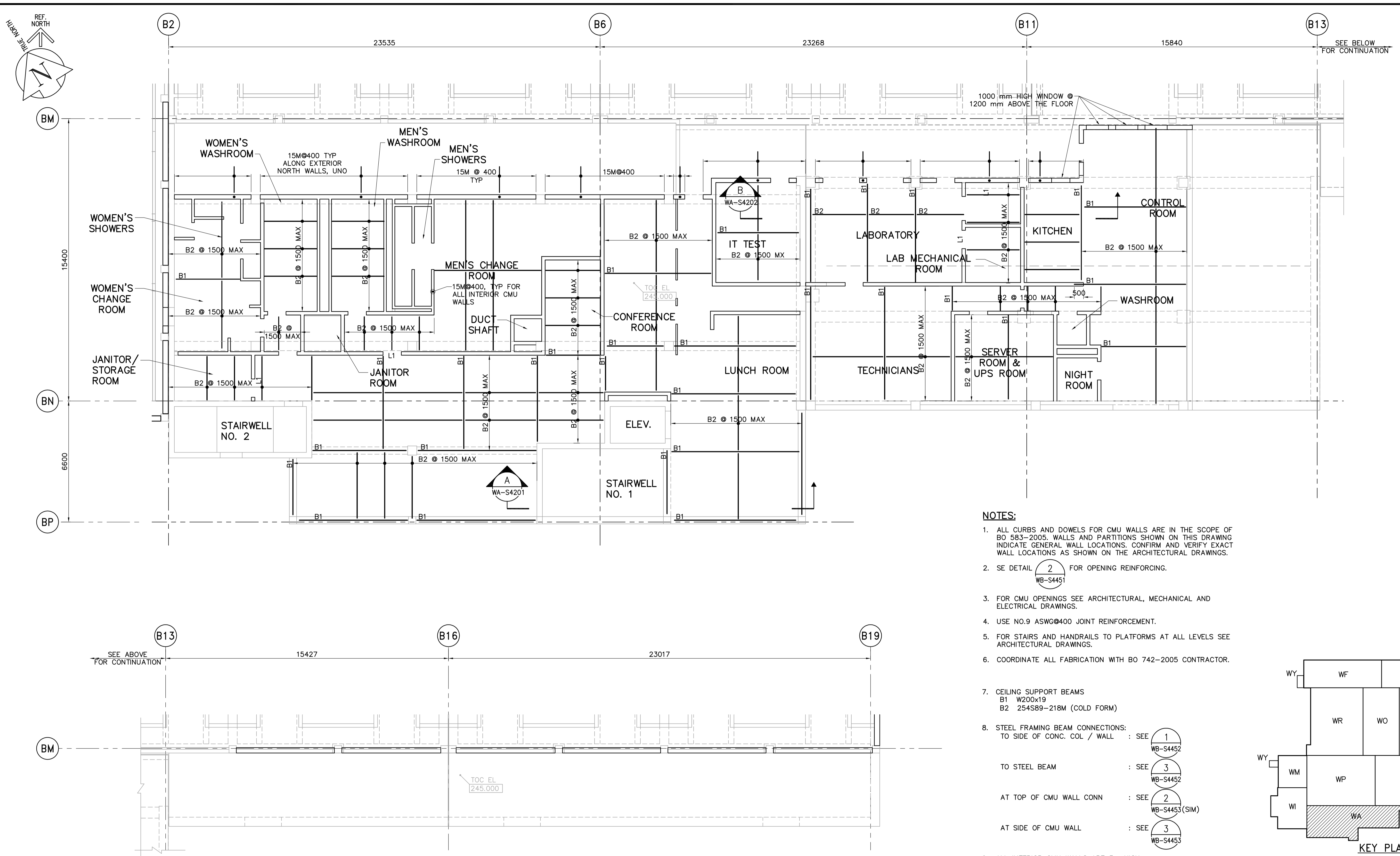
THIRD FLOOR PLAN 1:100
