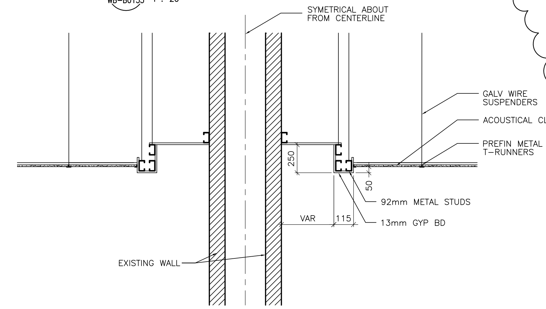
4 TYP CEILING DETAIL @ LIGHTING COVE WB-B0152 1 : 20
