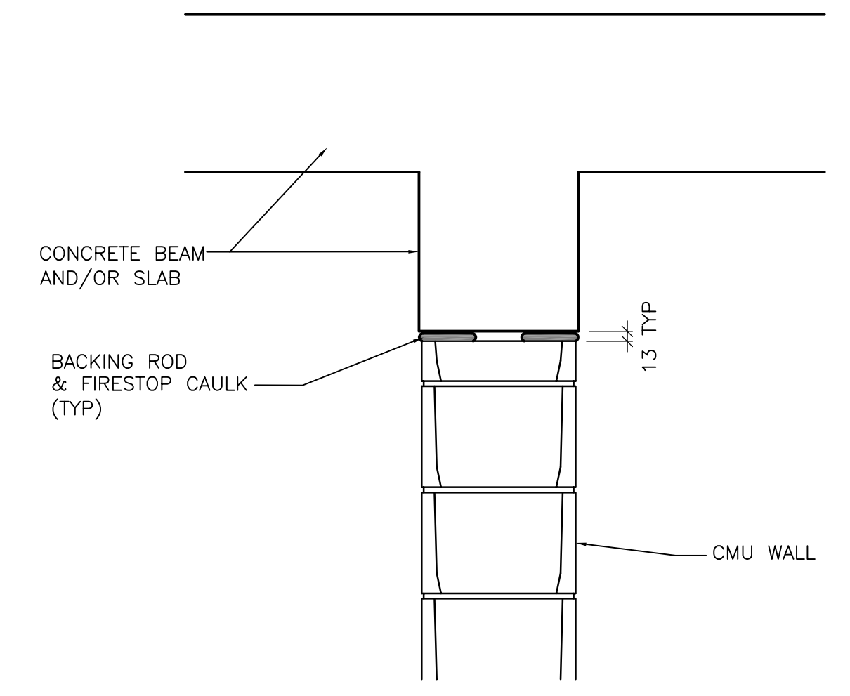
TYP DETAIL @ INTERIOR CMU WALLS 1 : 10
