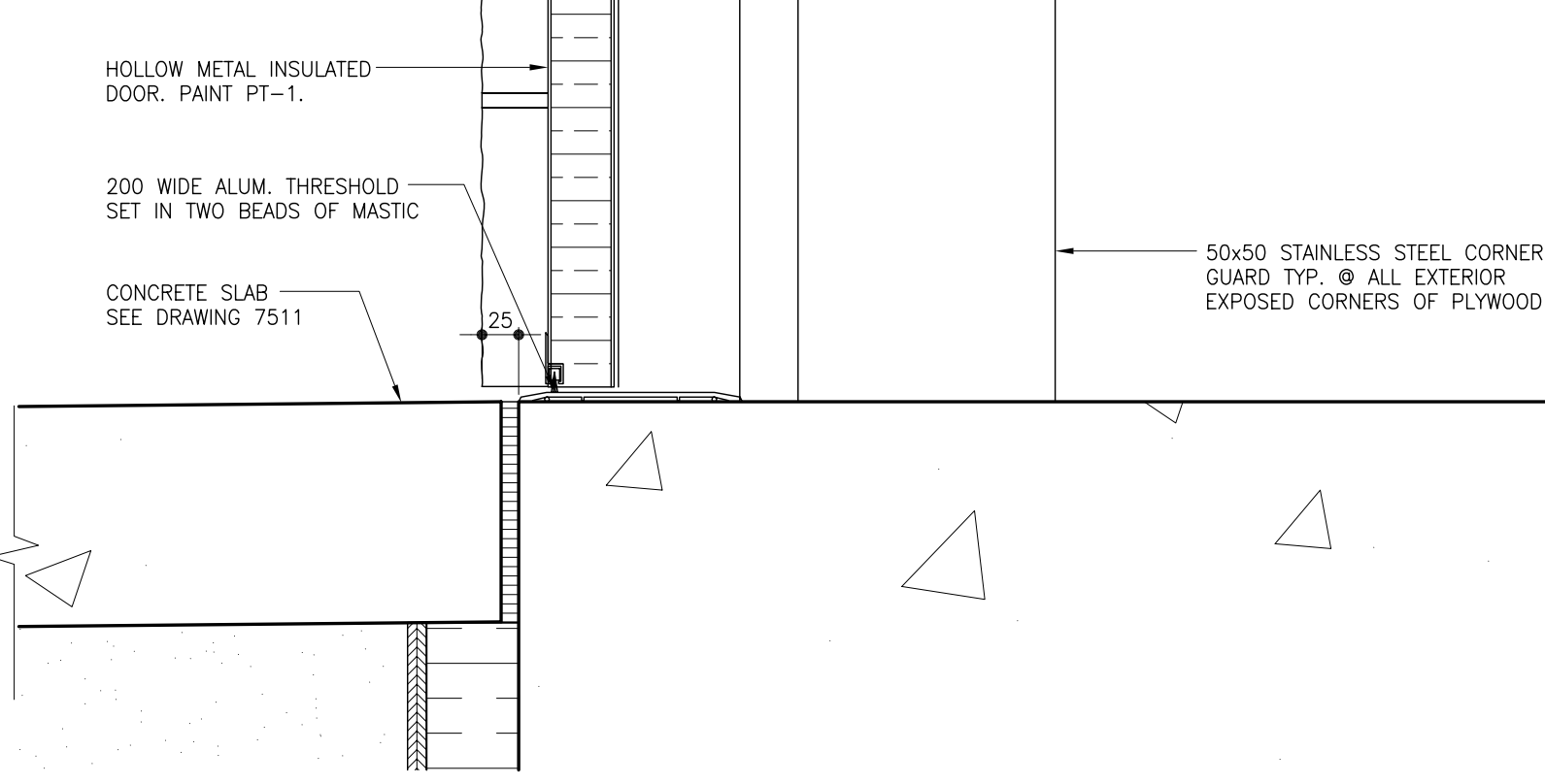
C THRESHOLD DETAIL B04 1:5
