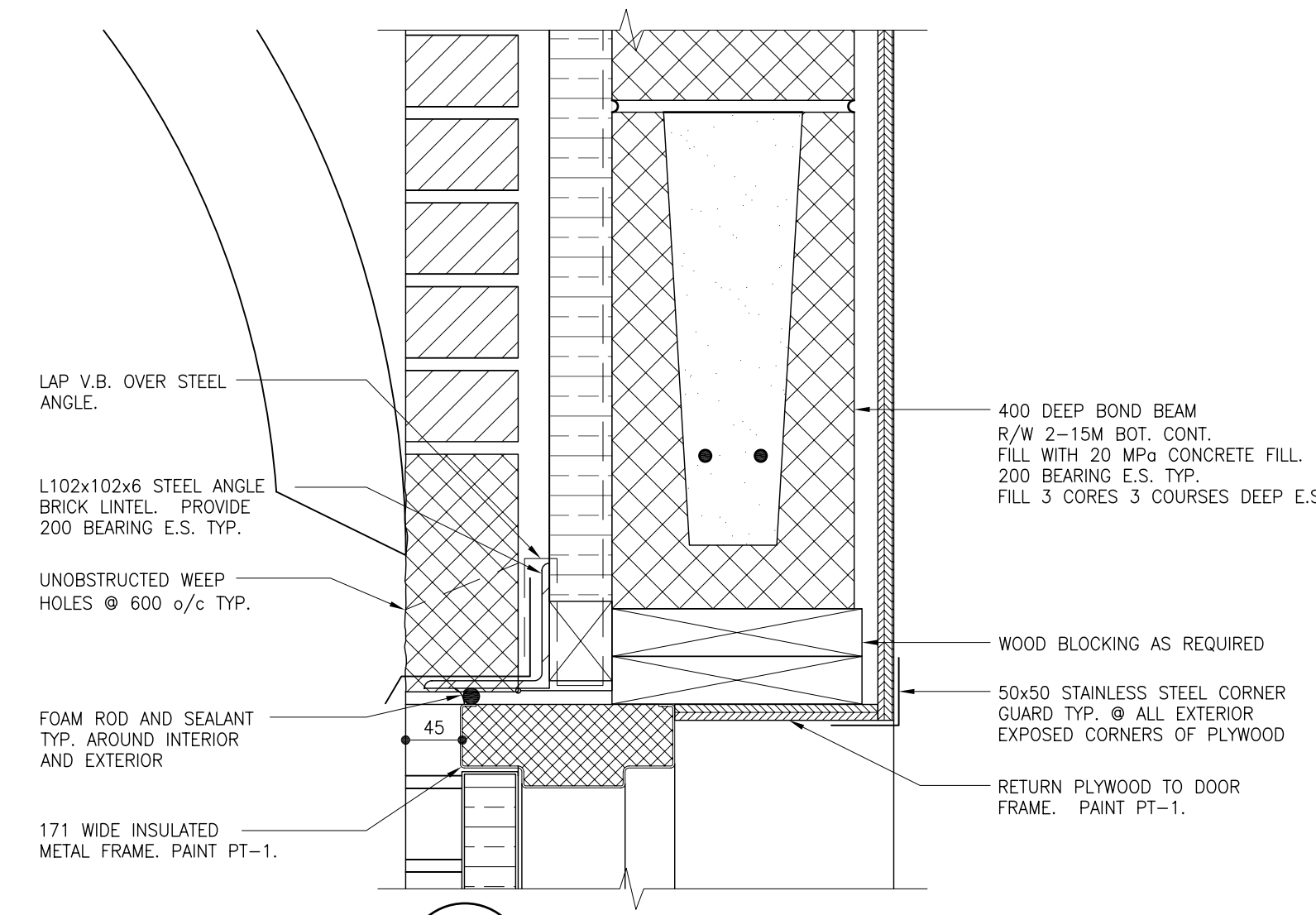
B LINTEL DETAIL B04 1:5
