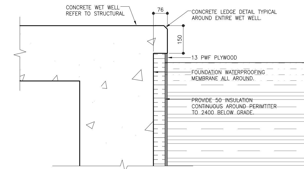
3 CONCRETE EDGE SECTION B04 1:10
