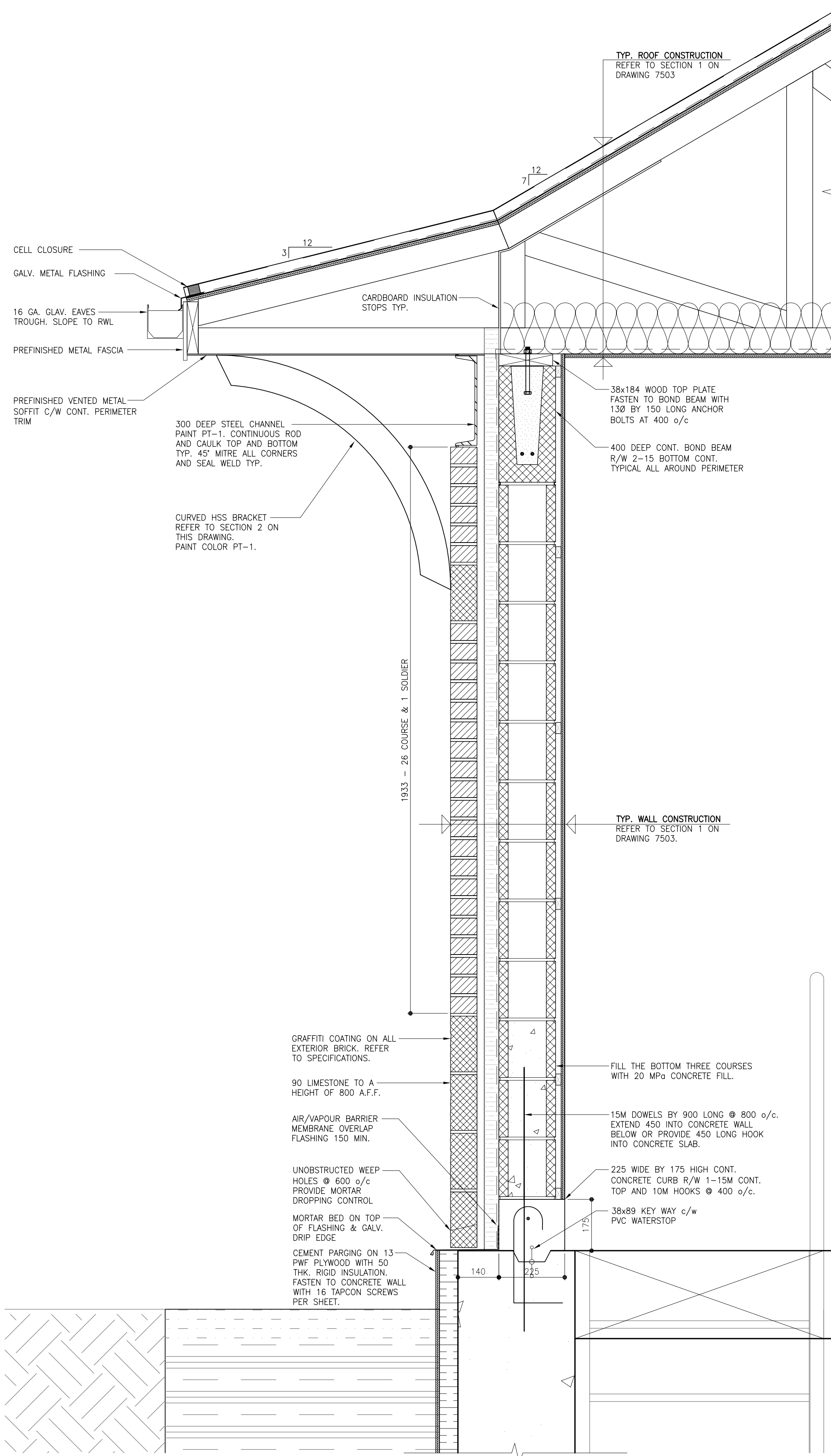
1 TYPICAL WALL SECTION B04 1:10
