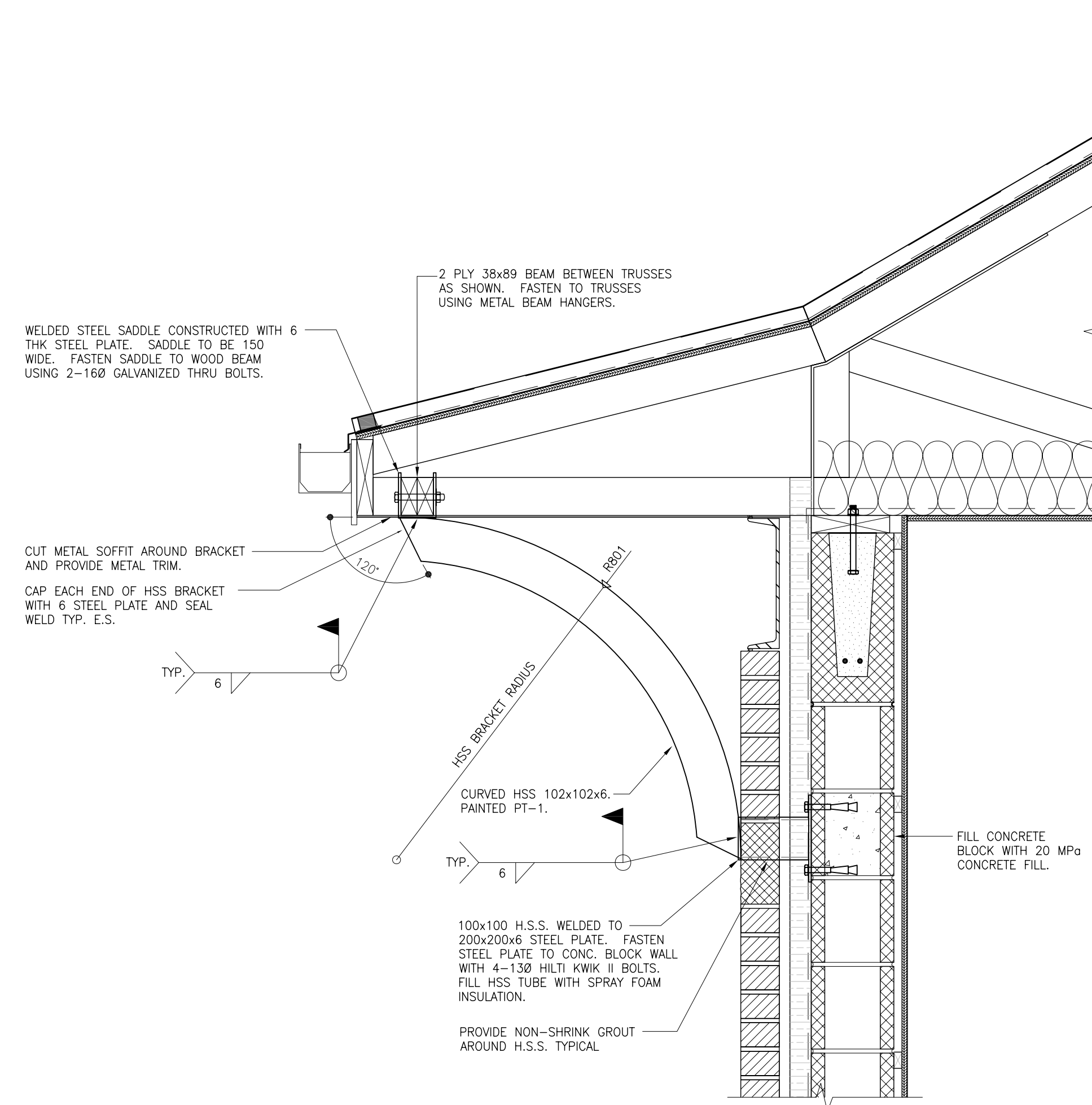
2 HSS BRACKET SECTION B04 1:10
