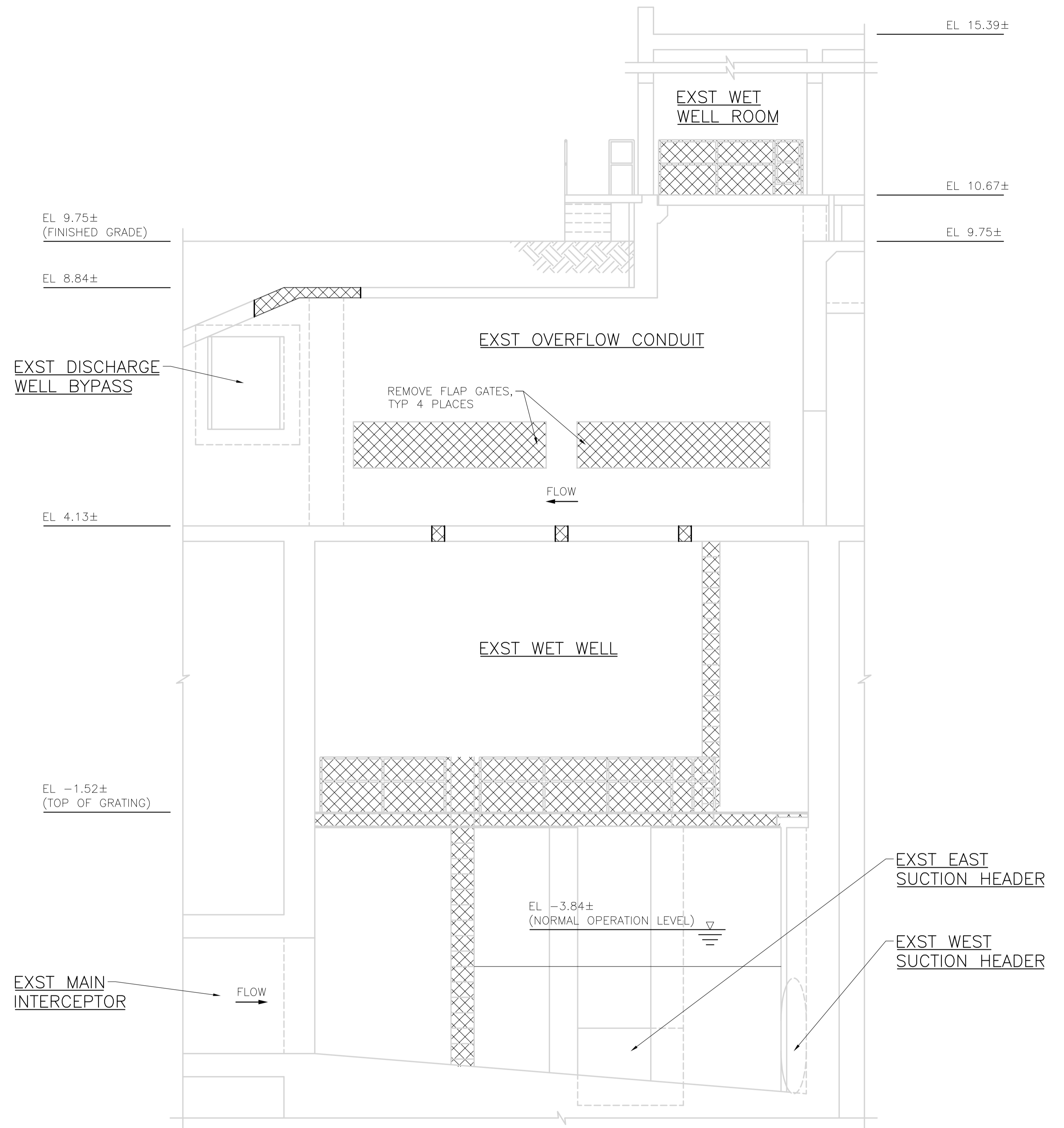
A SECTION 1:50 S0002
