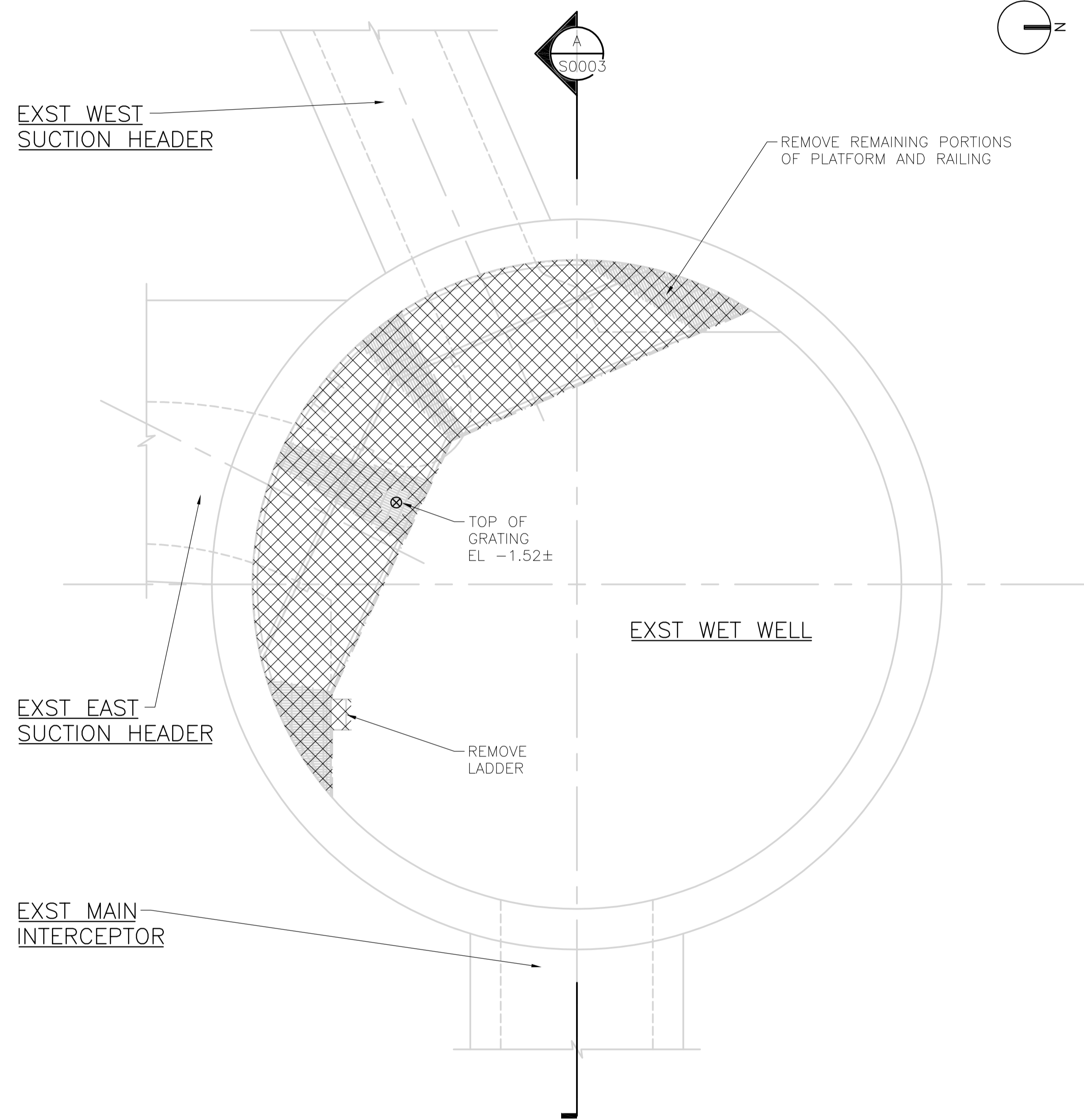
LOWER LEVEL PLAN ABOVE EL -1.52± 1:50
