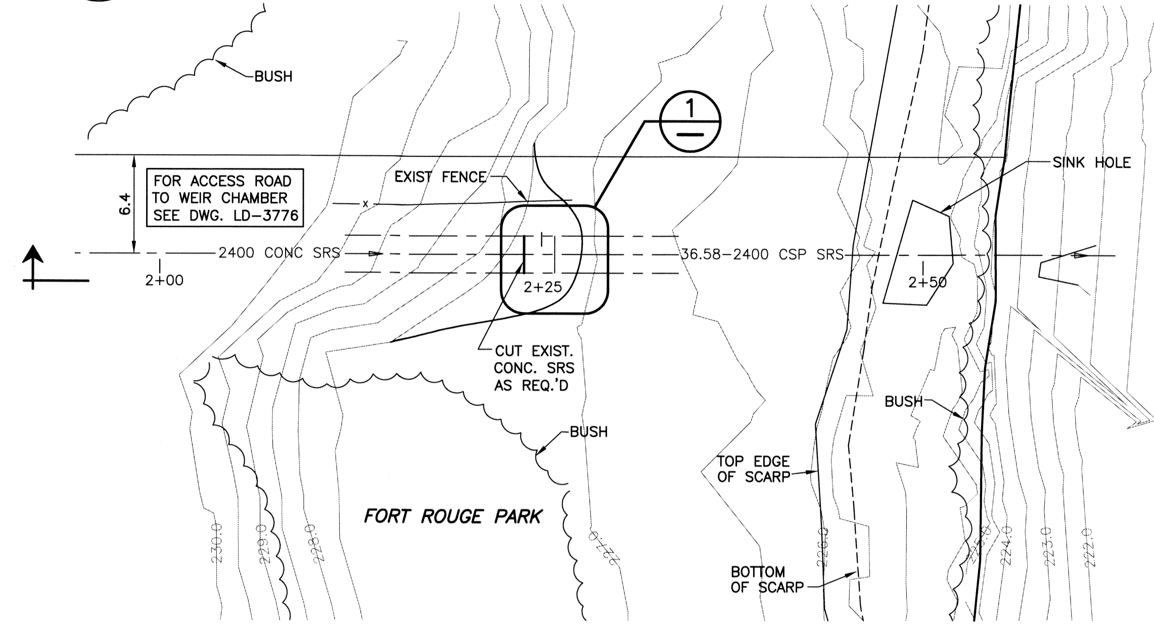
LOCATION PLAN SCALE: 1:250
