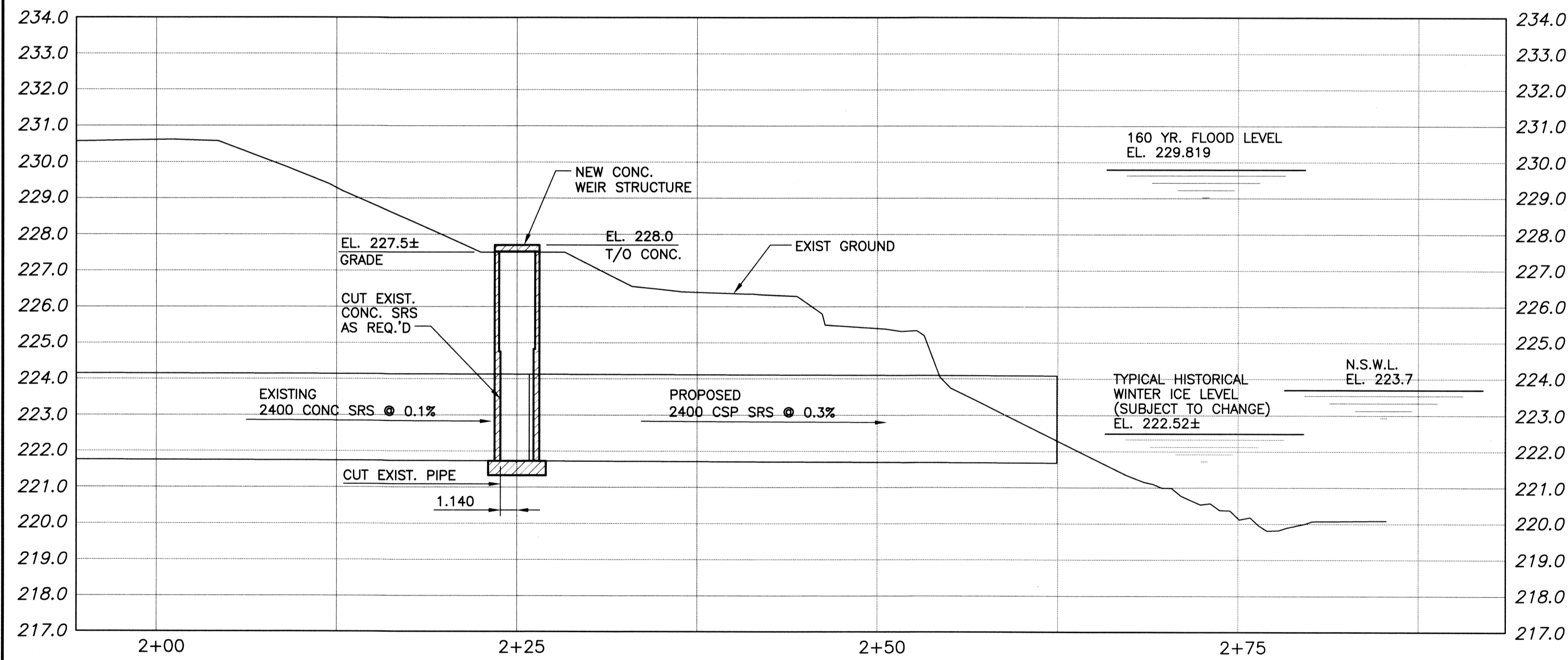
A SECTION - PROFILE SCALE: HOR 1:250 VER 1:100
