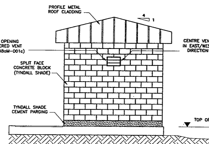
SOUTH ELEVATION SCALE: 1:40
