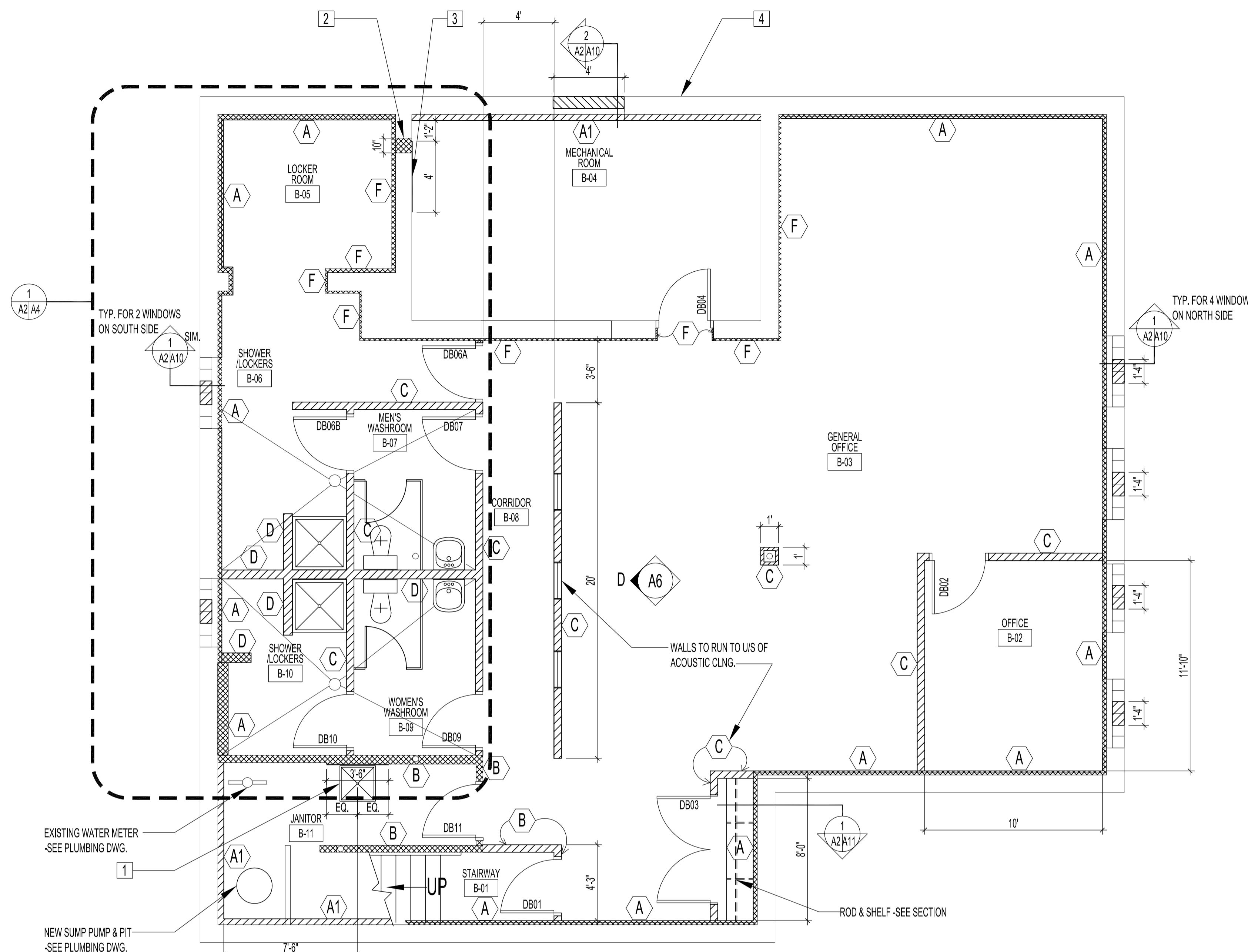
BASEMENT FLOOR PLAN - RENOVATION SCALE: 1/4"=1'-0"
