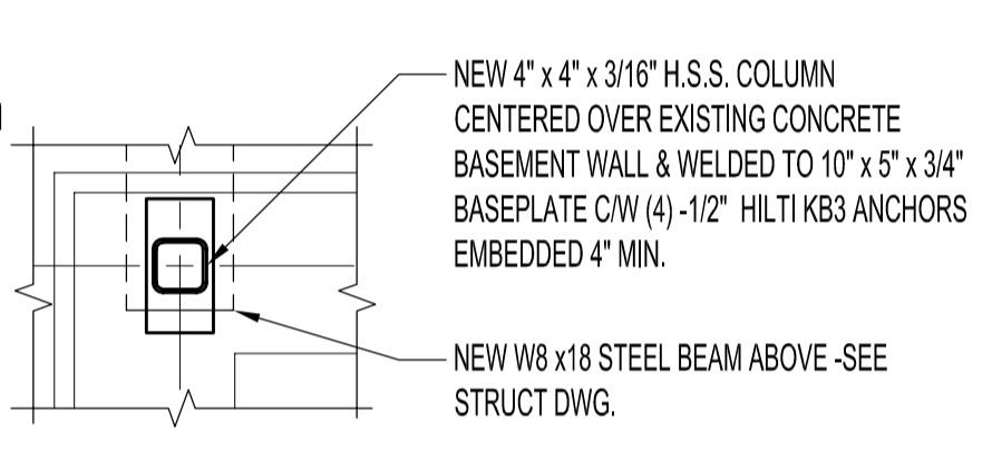
8 DETAIL - INTERIOR COLUMN BASE A3/A10 SCALE: 3/4"=1'-0"
