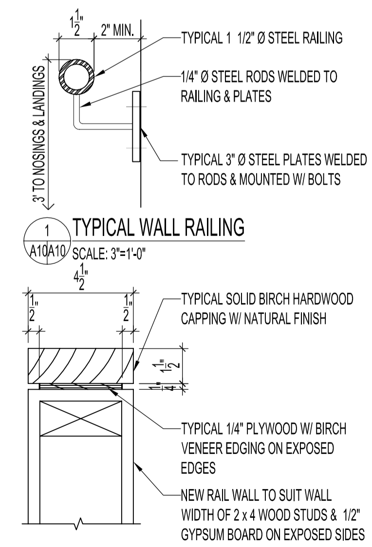
1 TYPICAL WALL RAILING A10A10 SCALE: 3"=1'-0"
