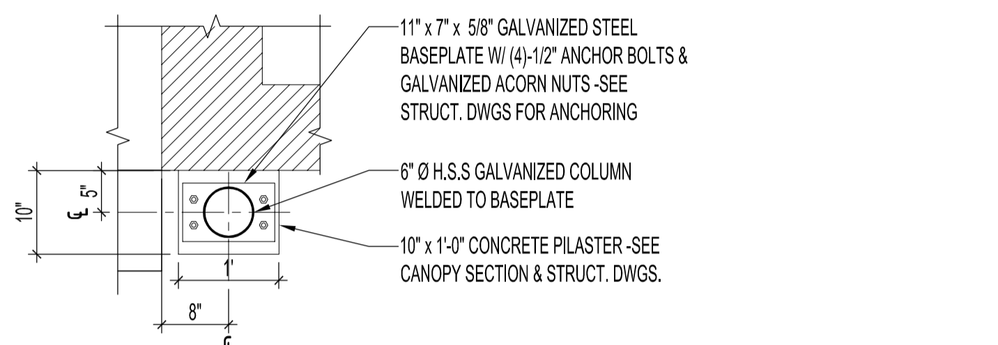
5 DETAIL - EXTERIOR COLUMN BASE A3/A10 SCALE: 3/4"=1'-0"
