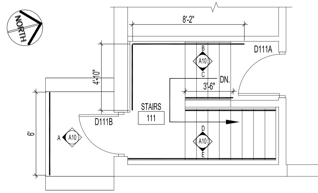
SOUTH EXIT STAIR & STAIRWAY 111 SCALE: 1/4"=1'-0"
