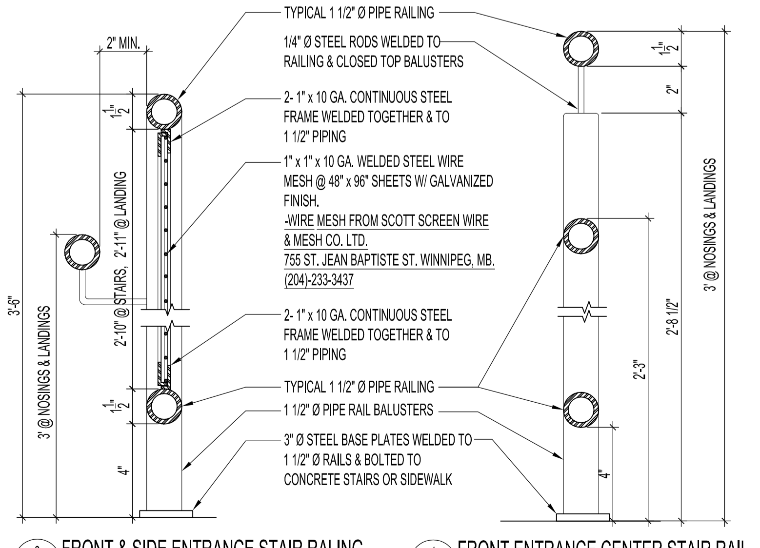
3 FRONT & SIDE ENTRANCE STAIR RAILING A10A10 SCALE: 3"=1'-0"
