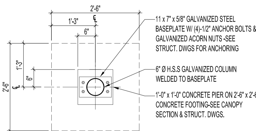
6 DETAIL - EXTERIOR COLUMN BASE A3/A10 SCALE: 3/4"=1'-0"
