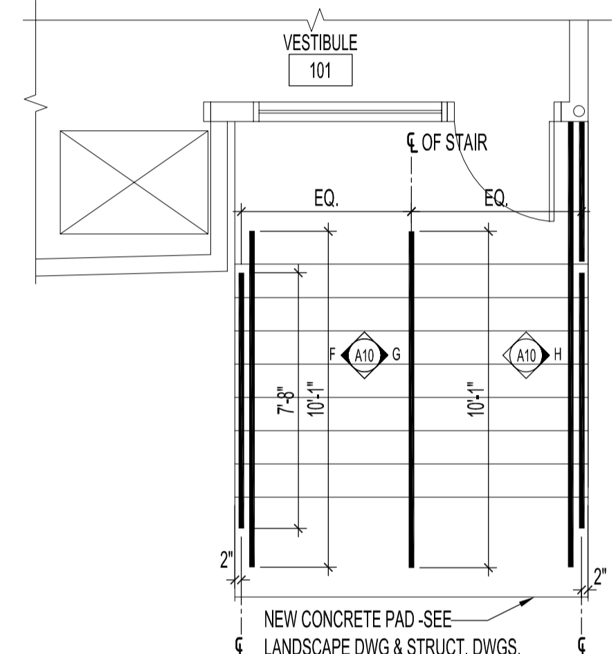
FRONT ENTRANCE STAIR SCALE: 1/4"=1'-0"
