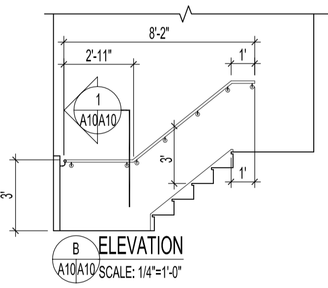
FRONT ENTRANCE STAIR SCALE: 1/4"=1'-0"
