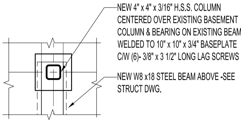
7 DETAIL - INTERIOR COLUMN BASE A3/A10 SCALE: 3/4"=1'-0"
