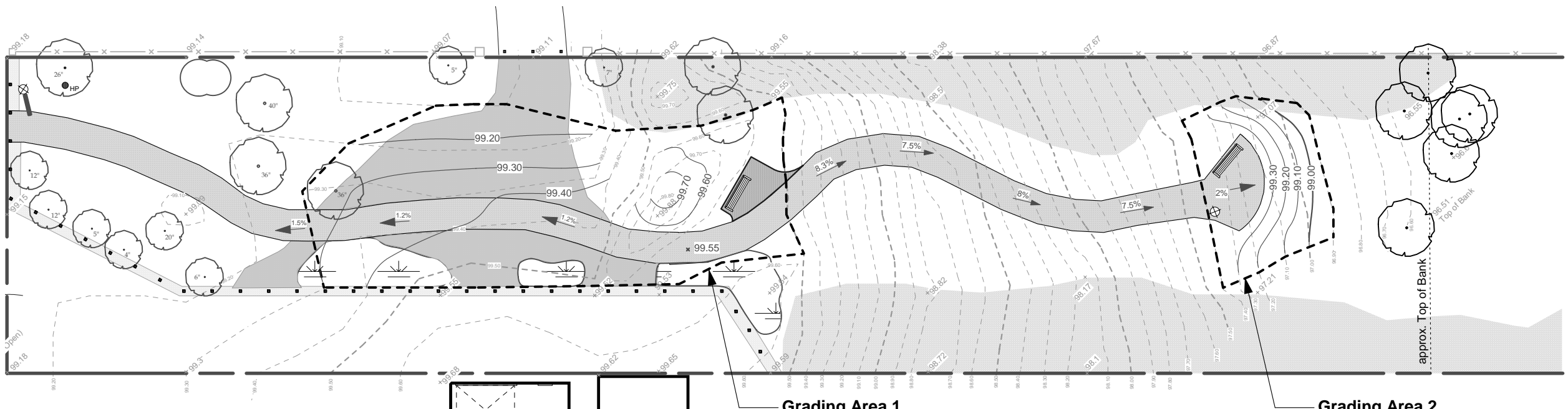
PROPOSED GRADING
