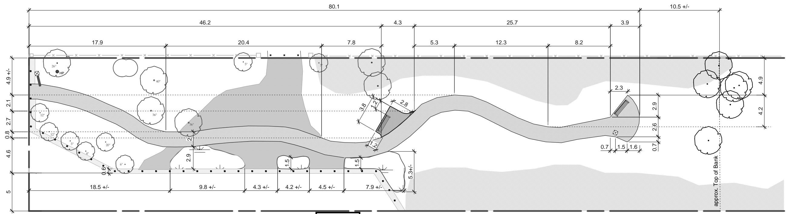
LAYOUT PLAN
