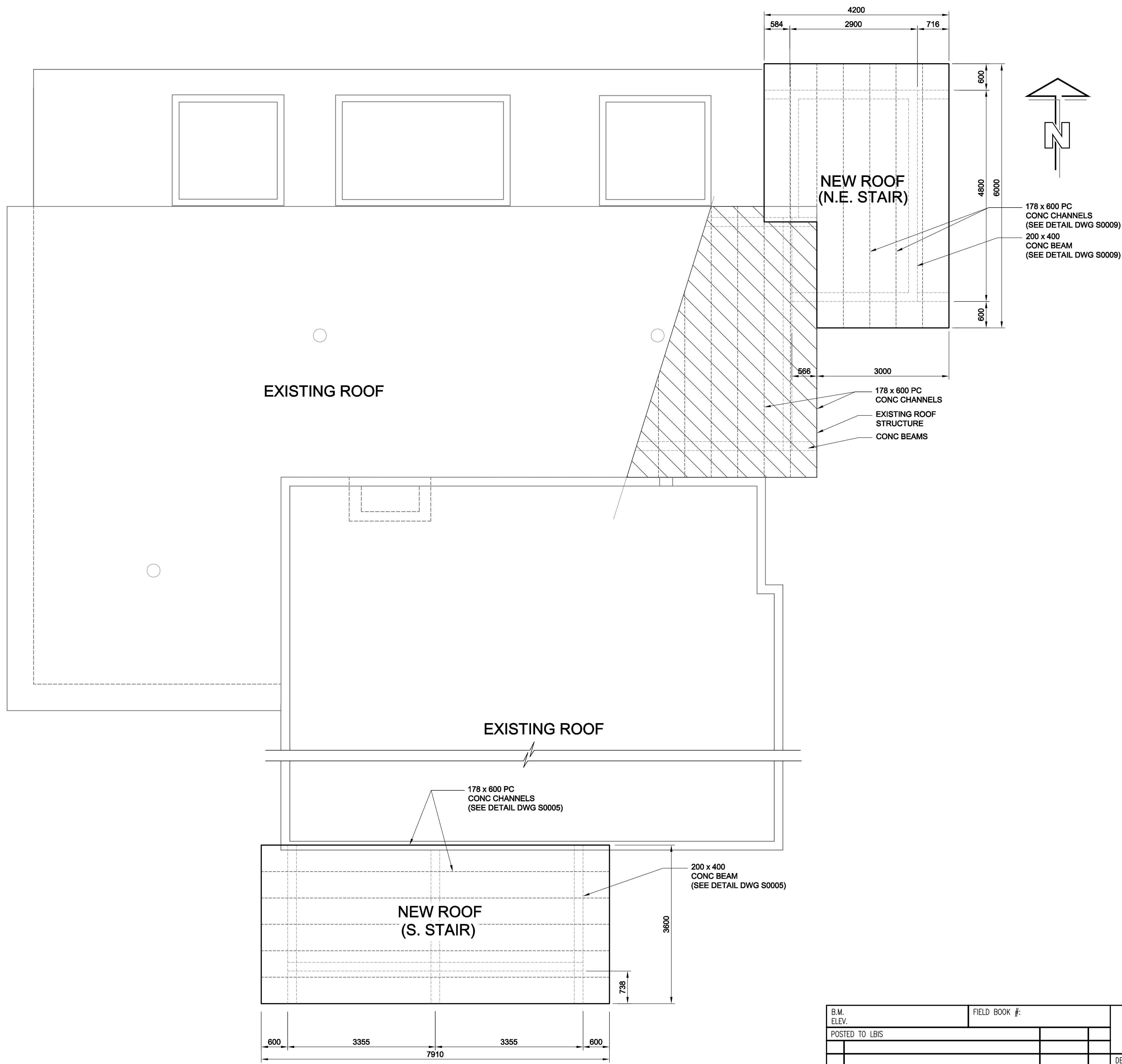
OVERALL ROOF PLAN SCALE 1:50 0 0.5 1 1.5 m
