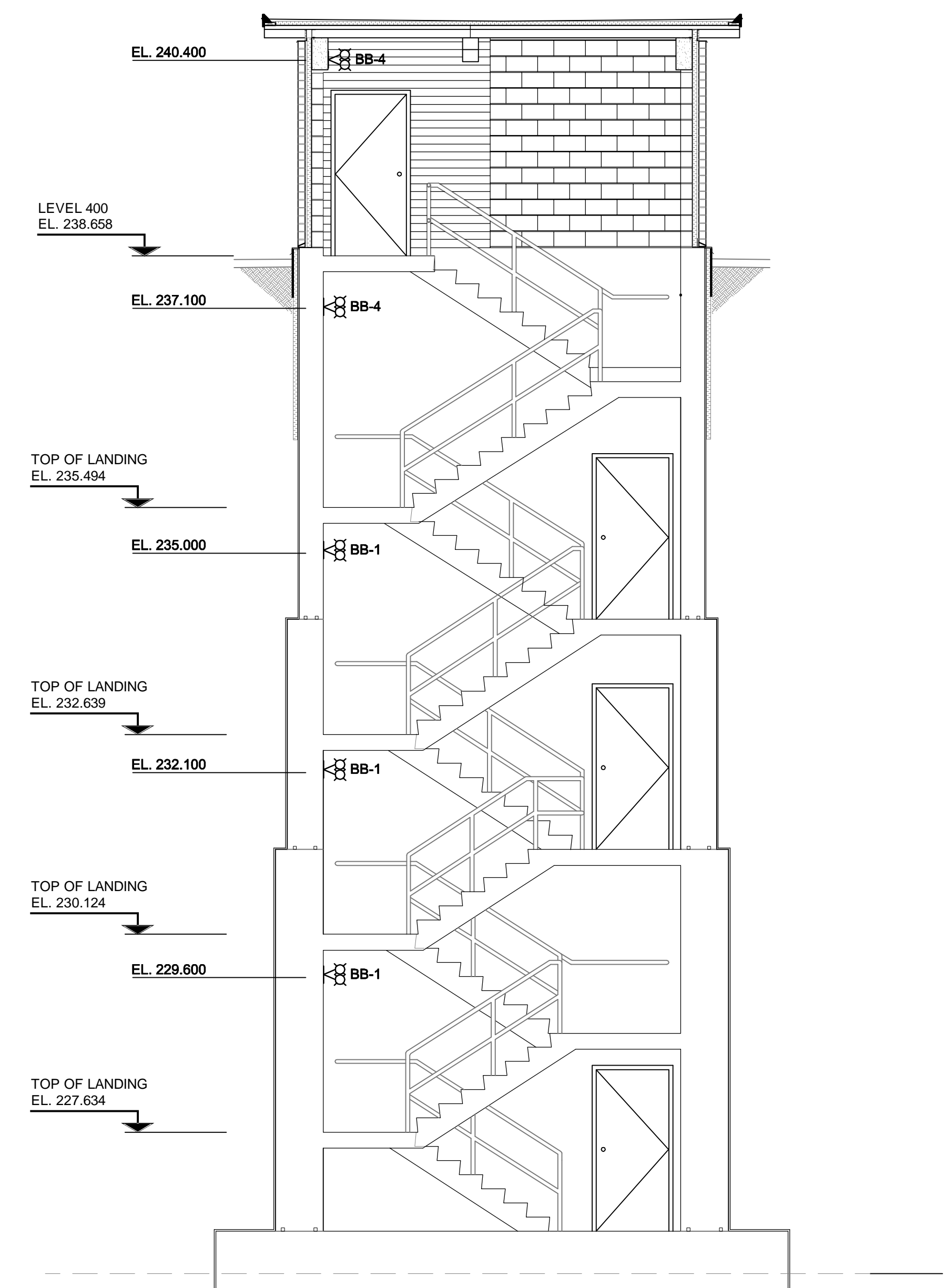
A STAIR SECTION - EMERGENCY LIGHTING SCALE: 1:50
