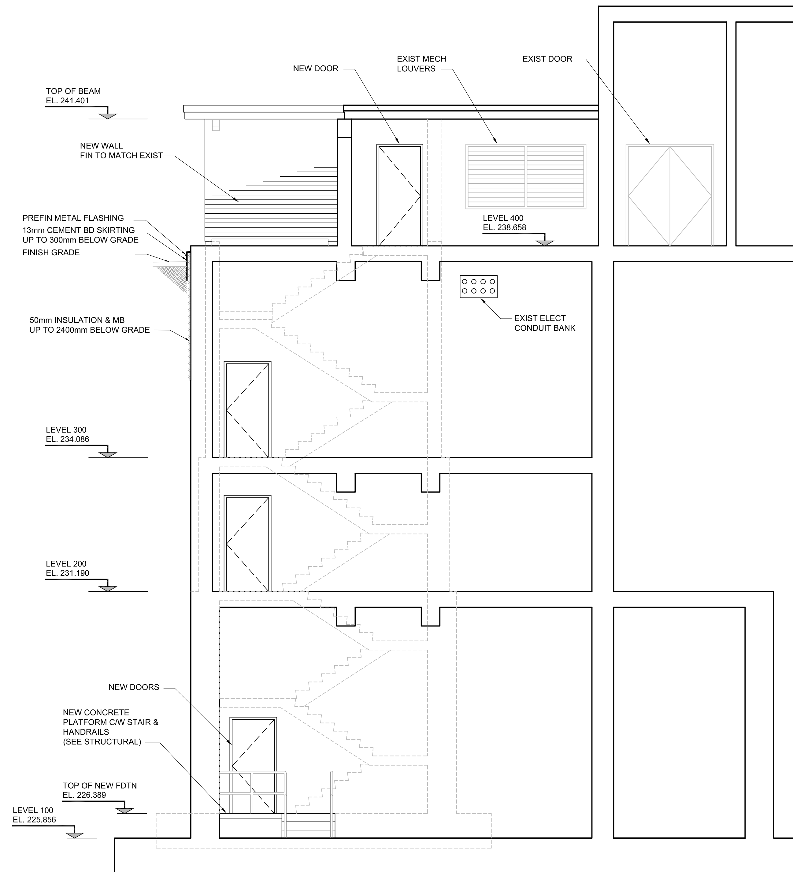
2 A05 BUILDING SECTION SCALE: 1:50
