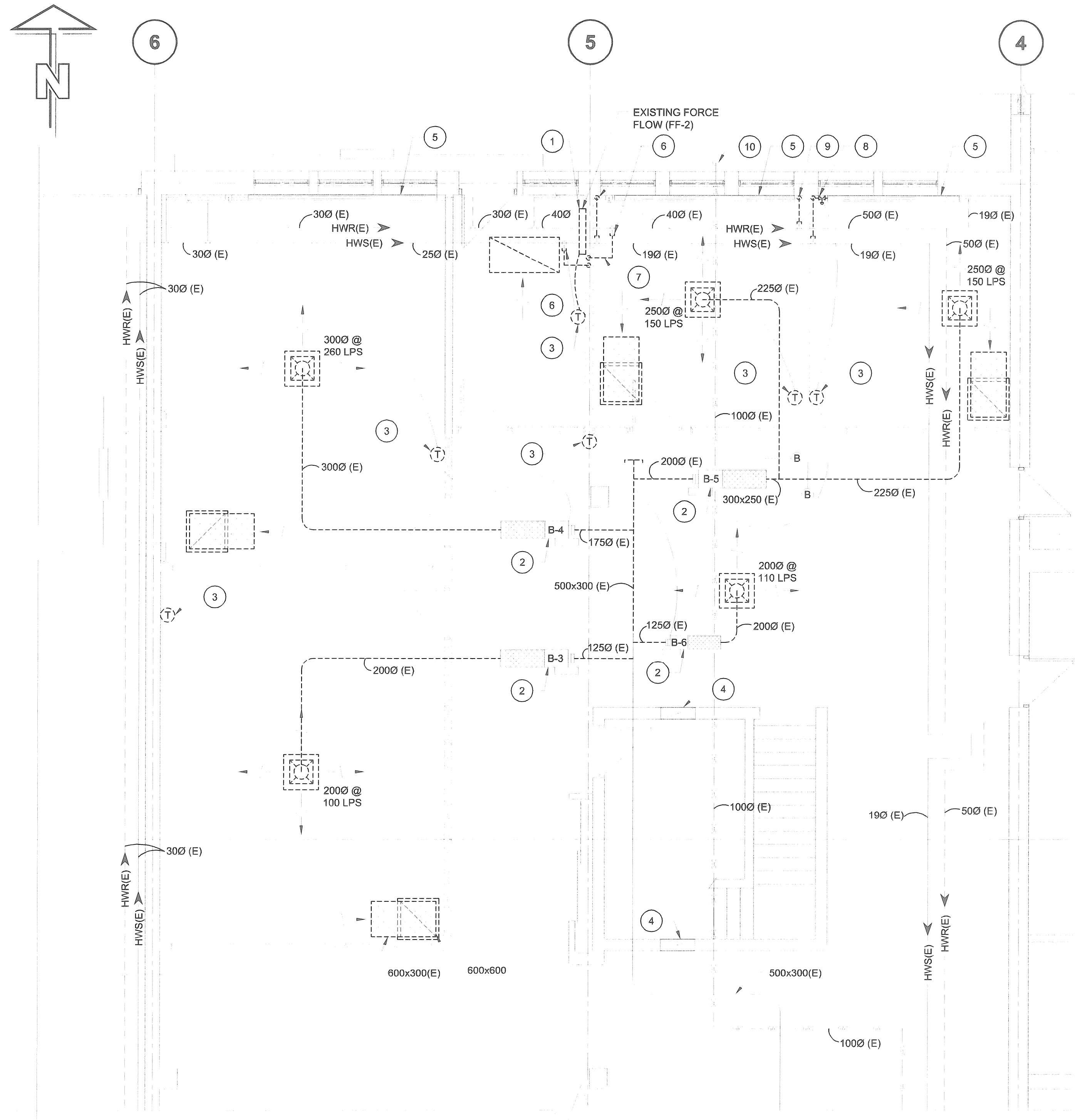
PLAN SCALE 1:50 MAIN FLOOR PLAN DEMOLITION
