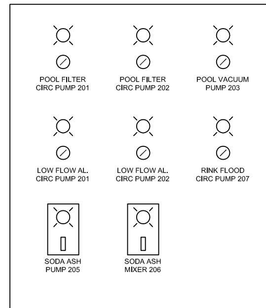
NEW CONTROL PANEL CP-101
