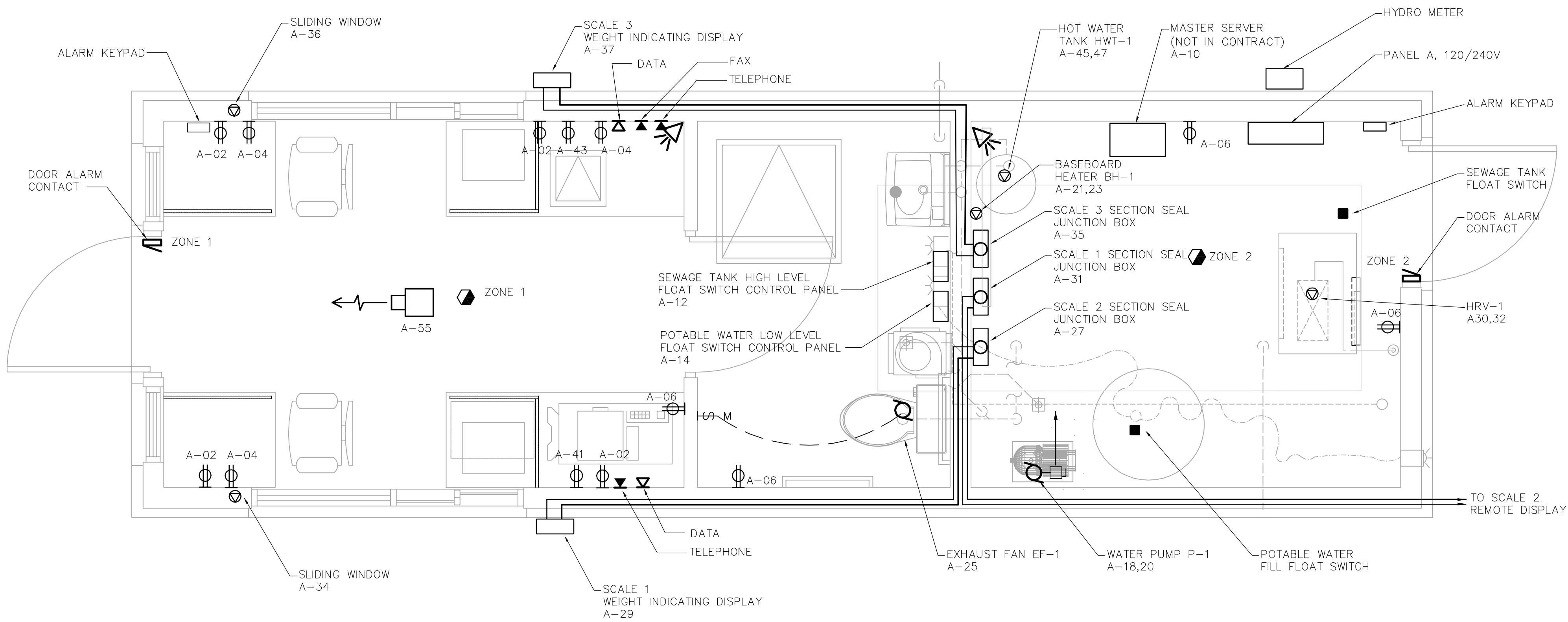
MAIN FLOOR POWER PLAN 1:20
