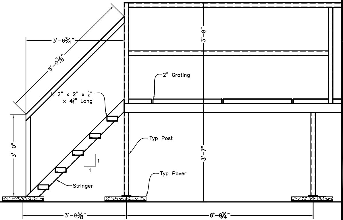
Typical Stair Detail Scale: 1/2" = 1'-0"
