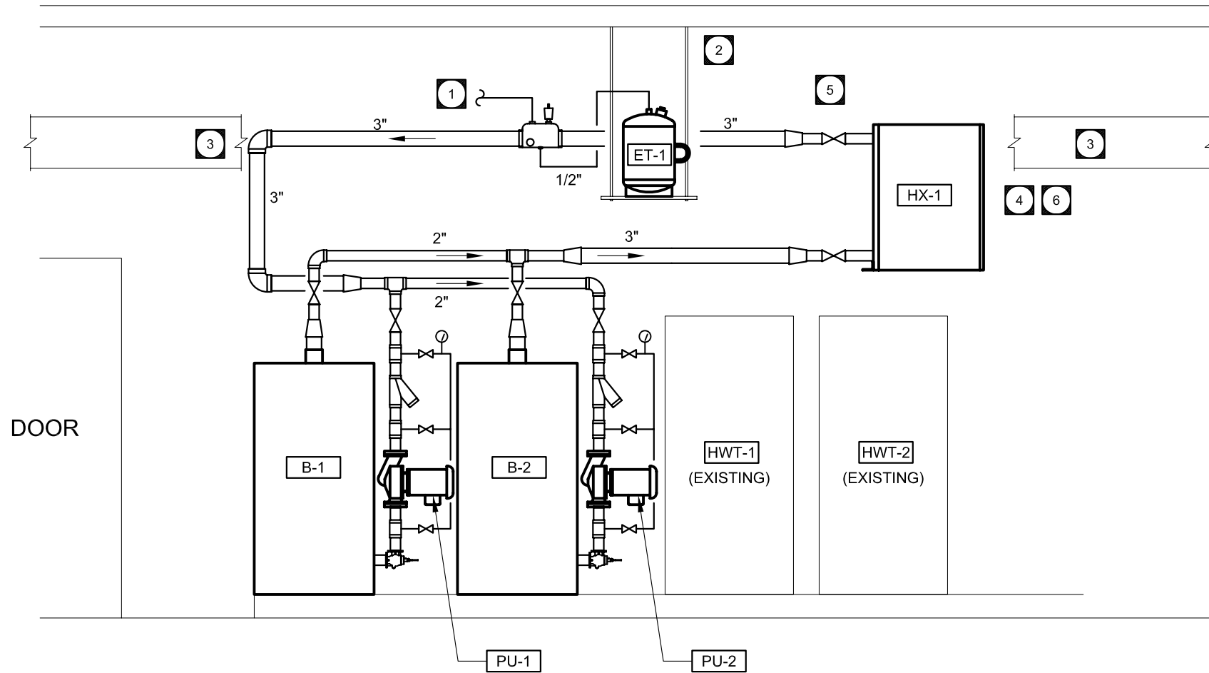
1 EQUIPMENT ROOM SECTION M2 SCALE: 3/8" = 1'-0"
