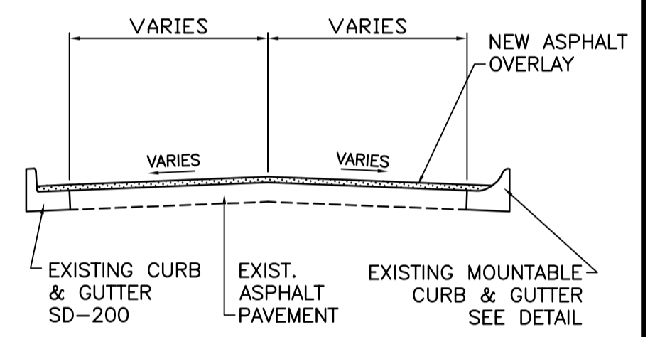
ASPHALT ROAD WITH CONCRETE CURB & GUTTER N.T.S.
