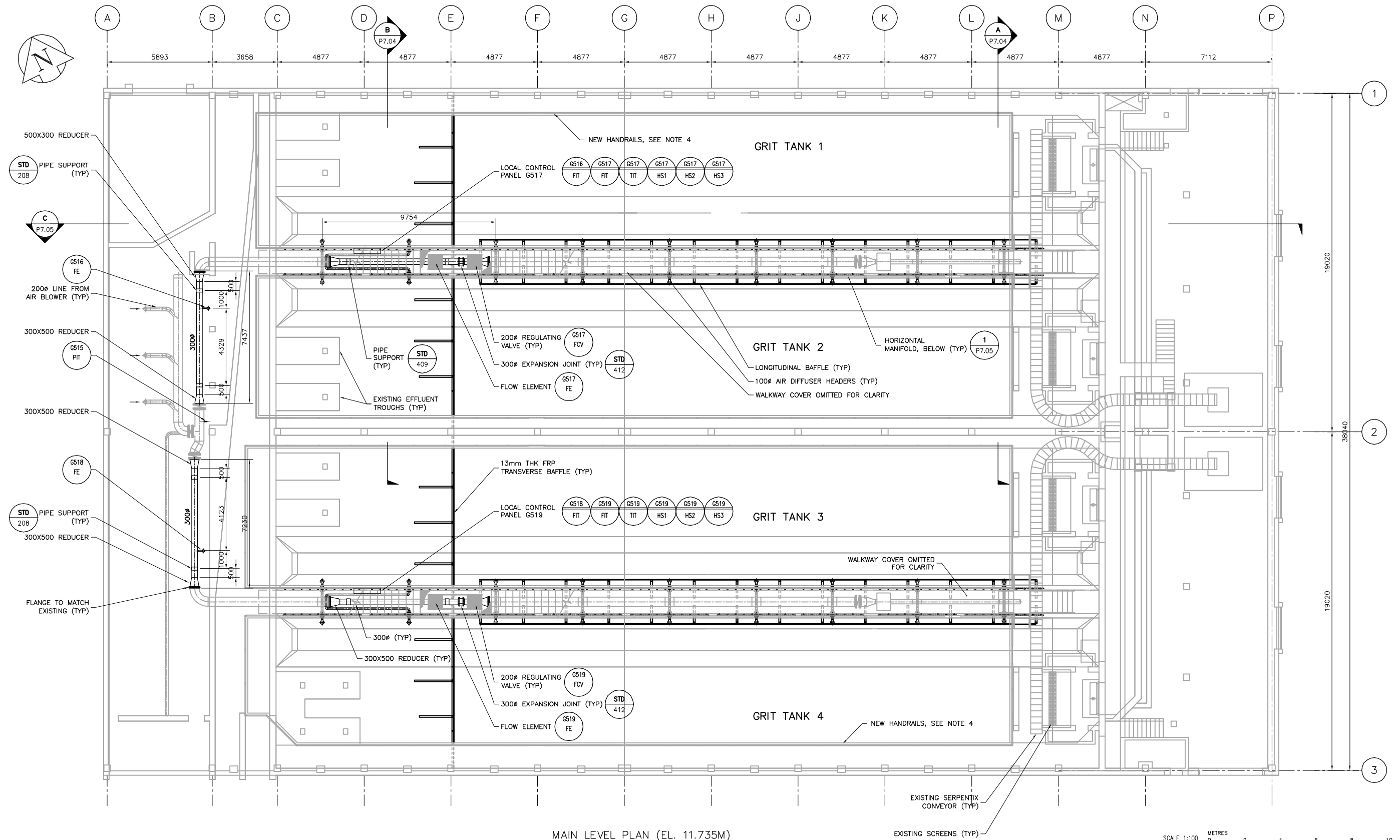
MAIN LEVEL PLAN (EL. 11.735M) SCALE 1:100
