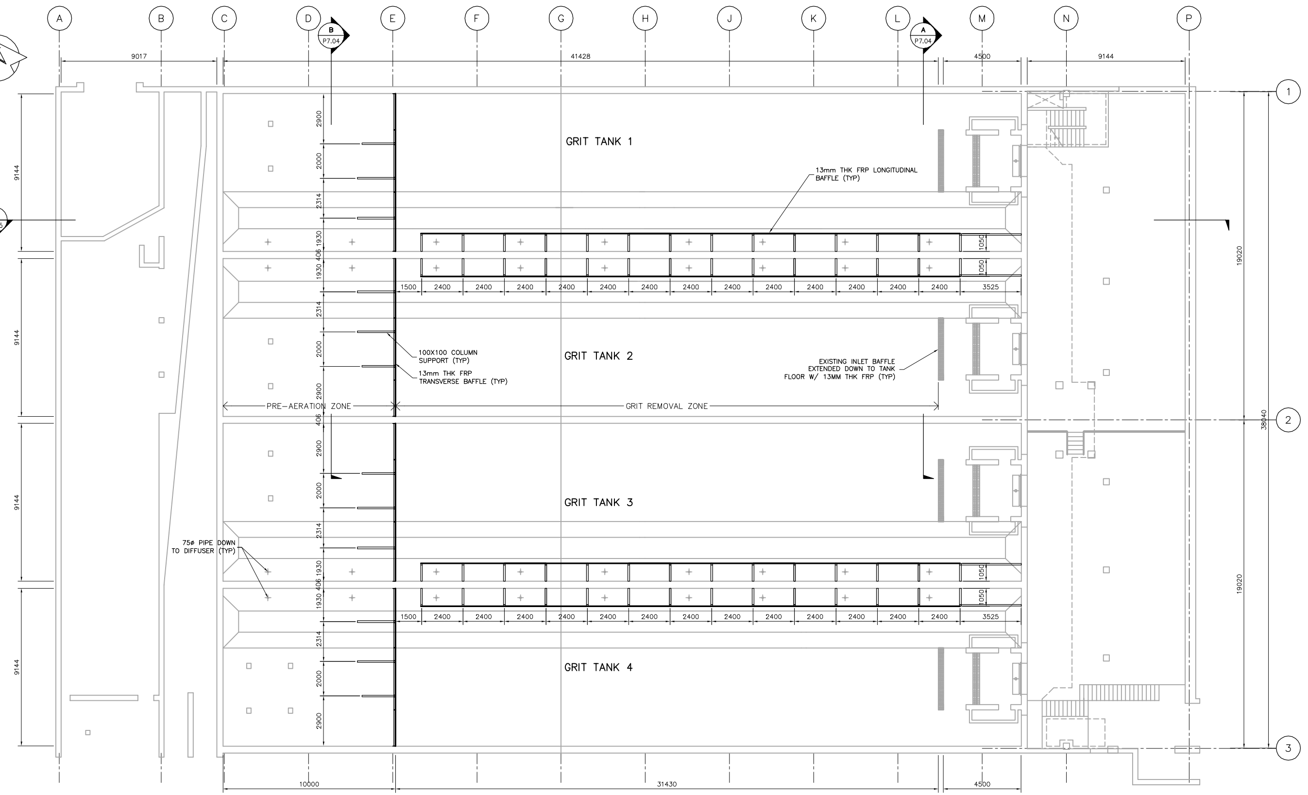
GRIT TANK BAFFLE LOWER LEVEL PLAN (EL. 9.601M) SCALE 1:100
