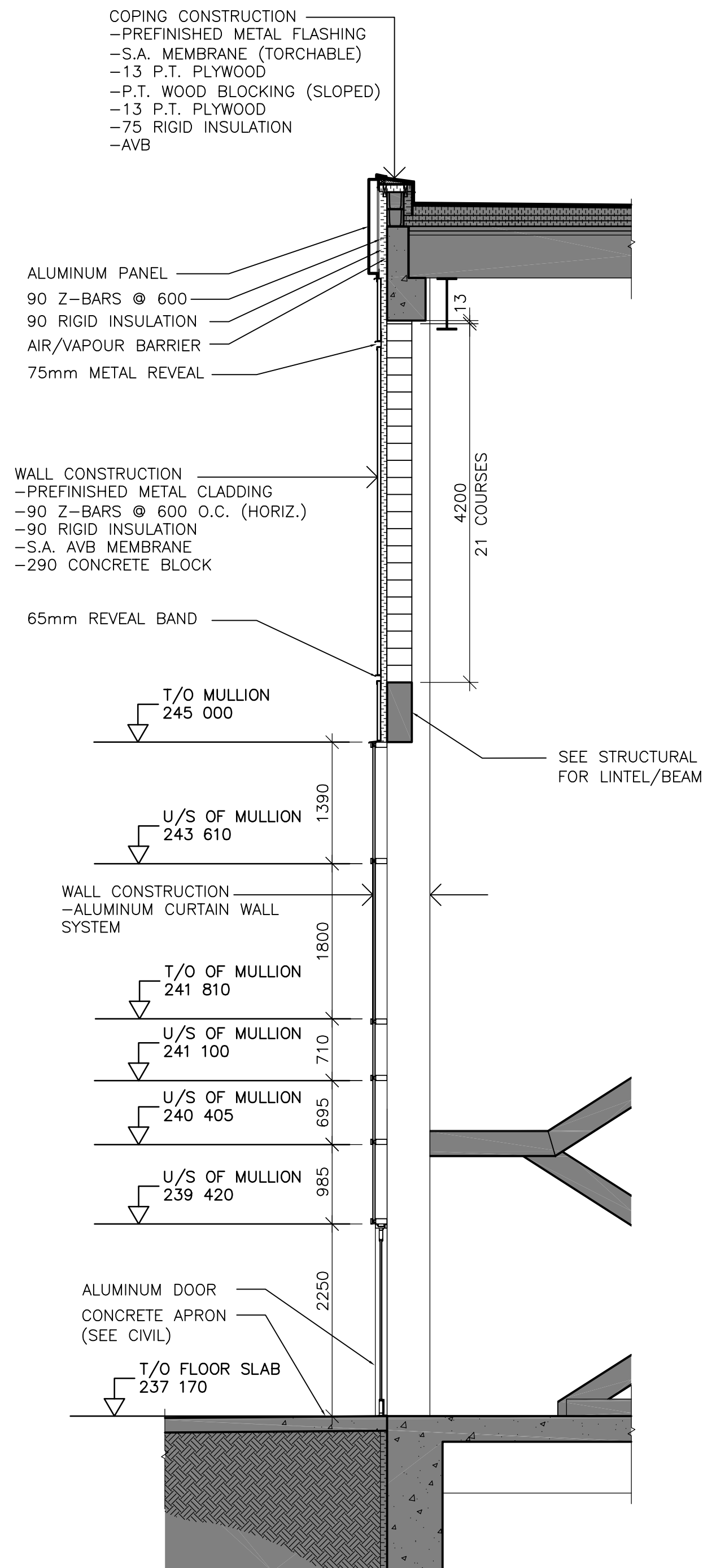
13 WALL SECTION WB-B0110 1 : 50
