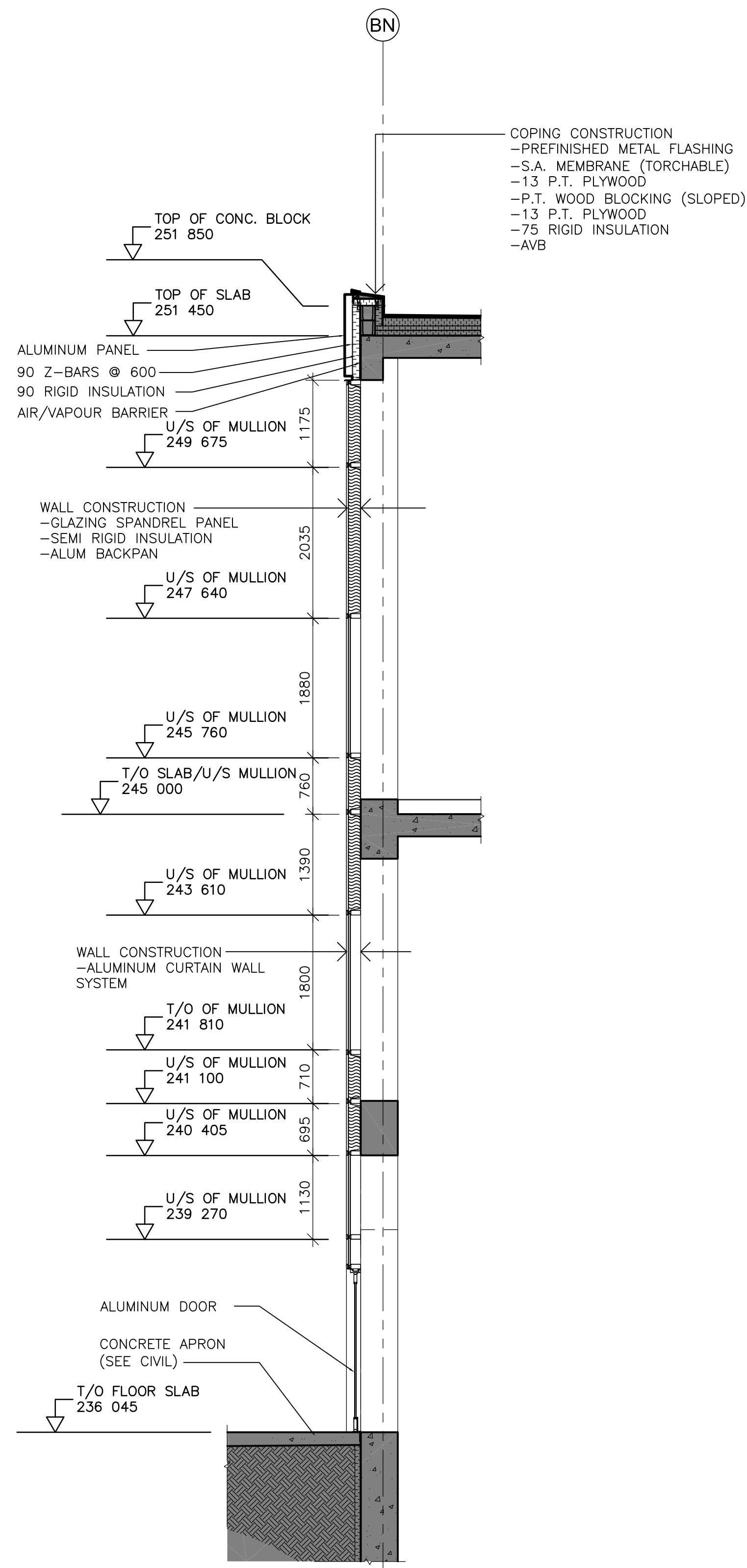
12 WALL SECTION WB-B0110 1 : 50
