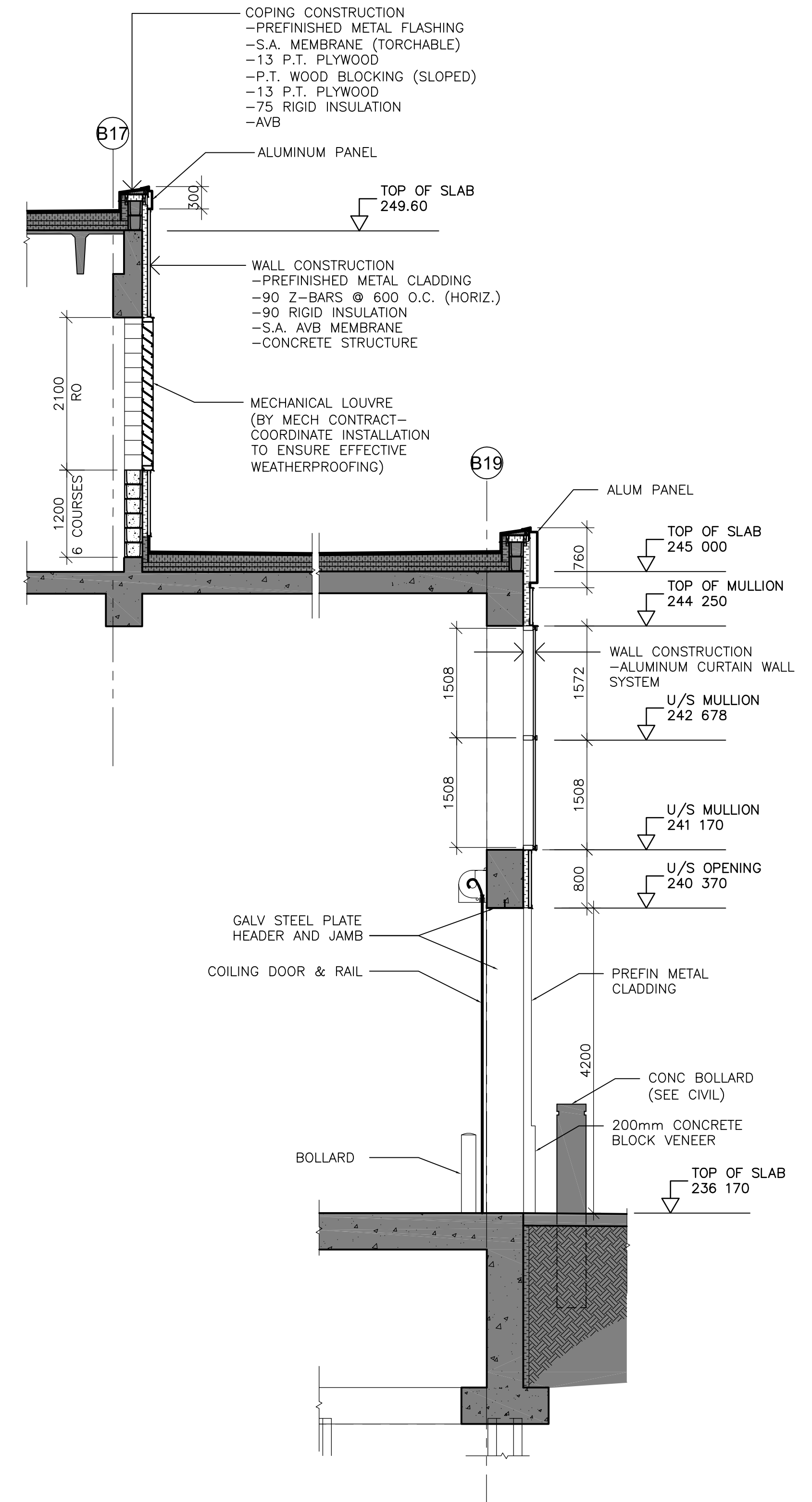
14 WALL SECTION WB-B0110 1 : 50
