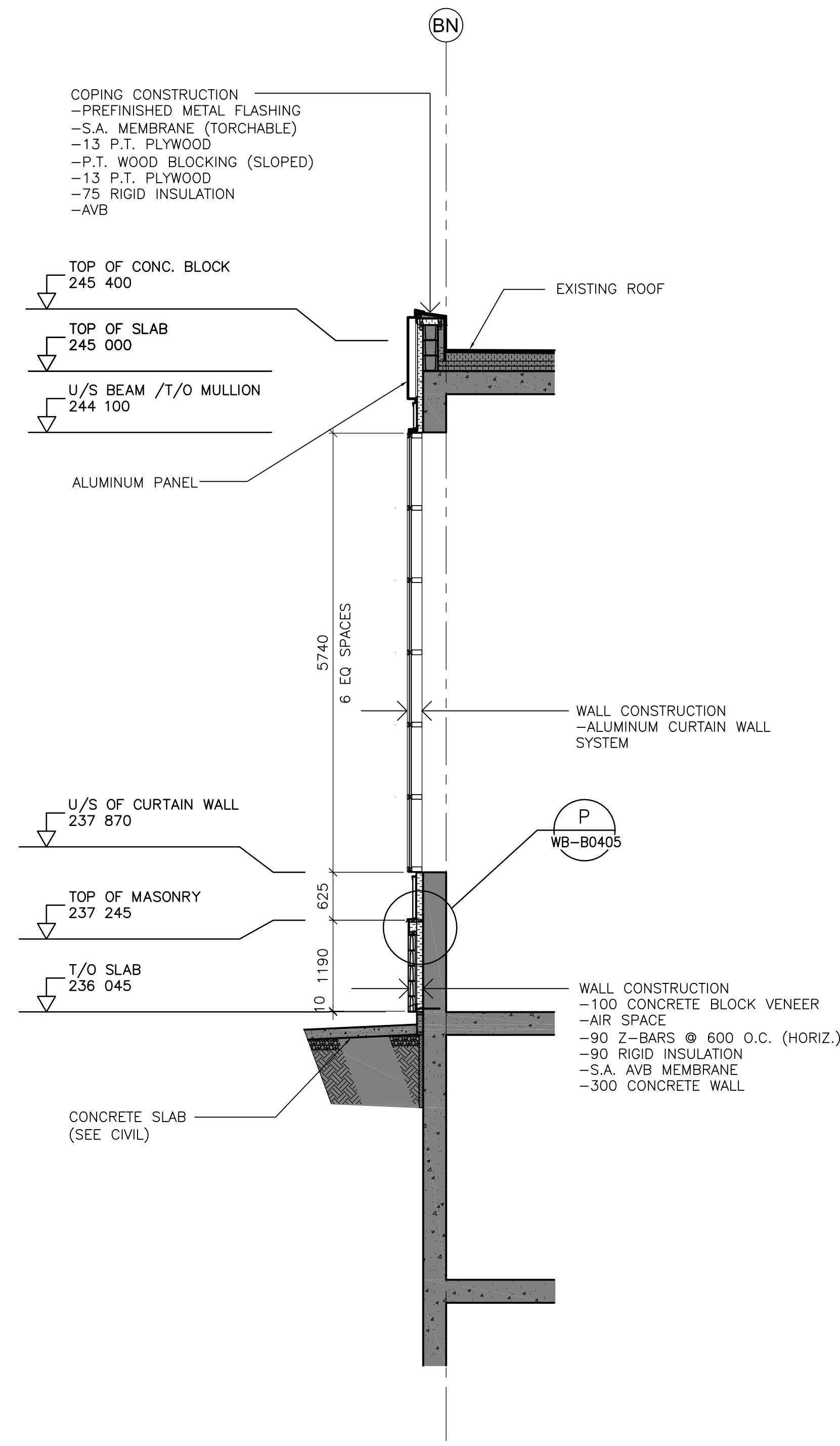
10 WALL SECTION WB-B0110 1 : 50
