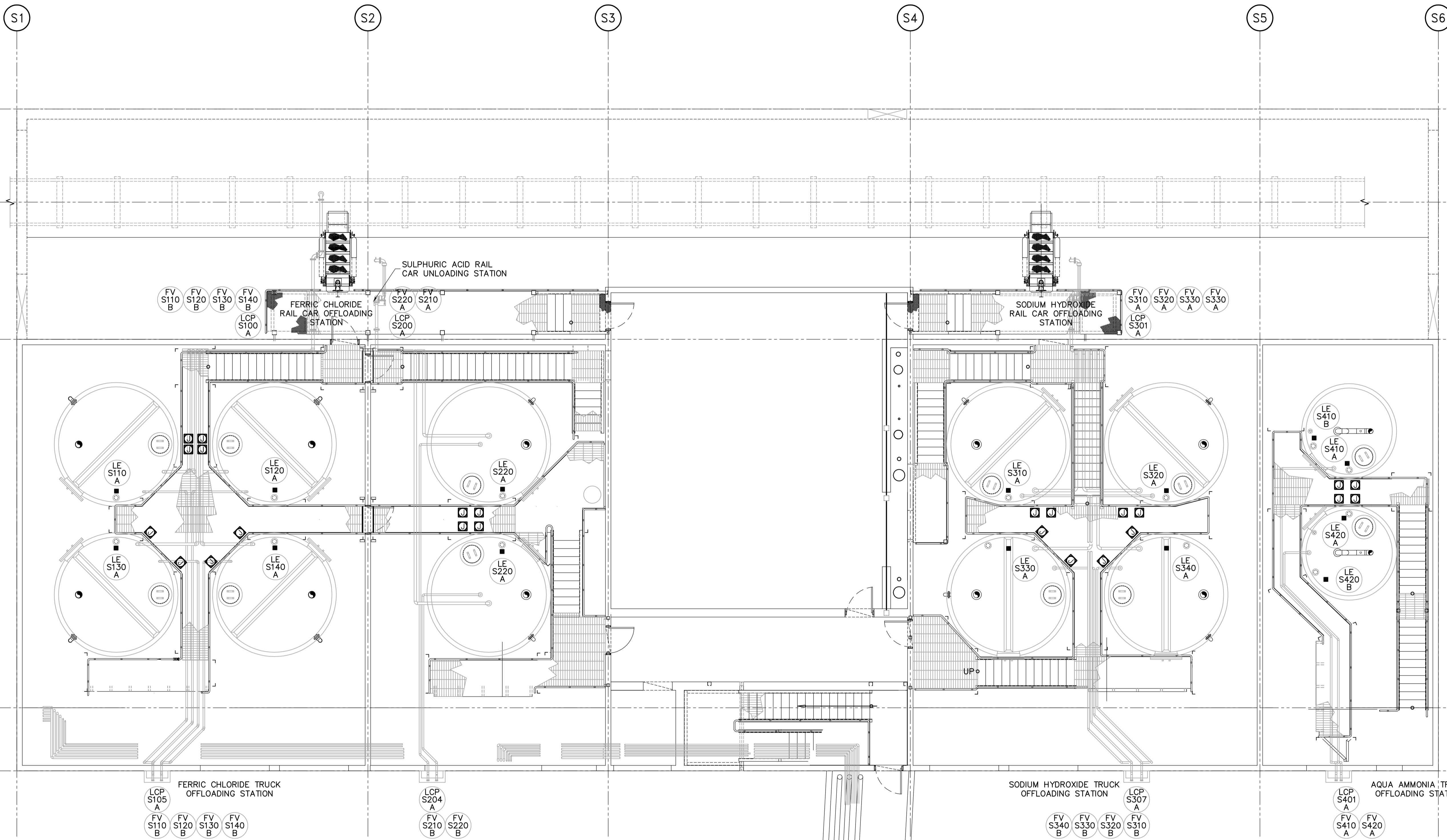
CATWALK PLAN
