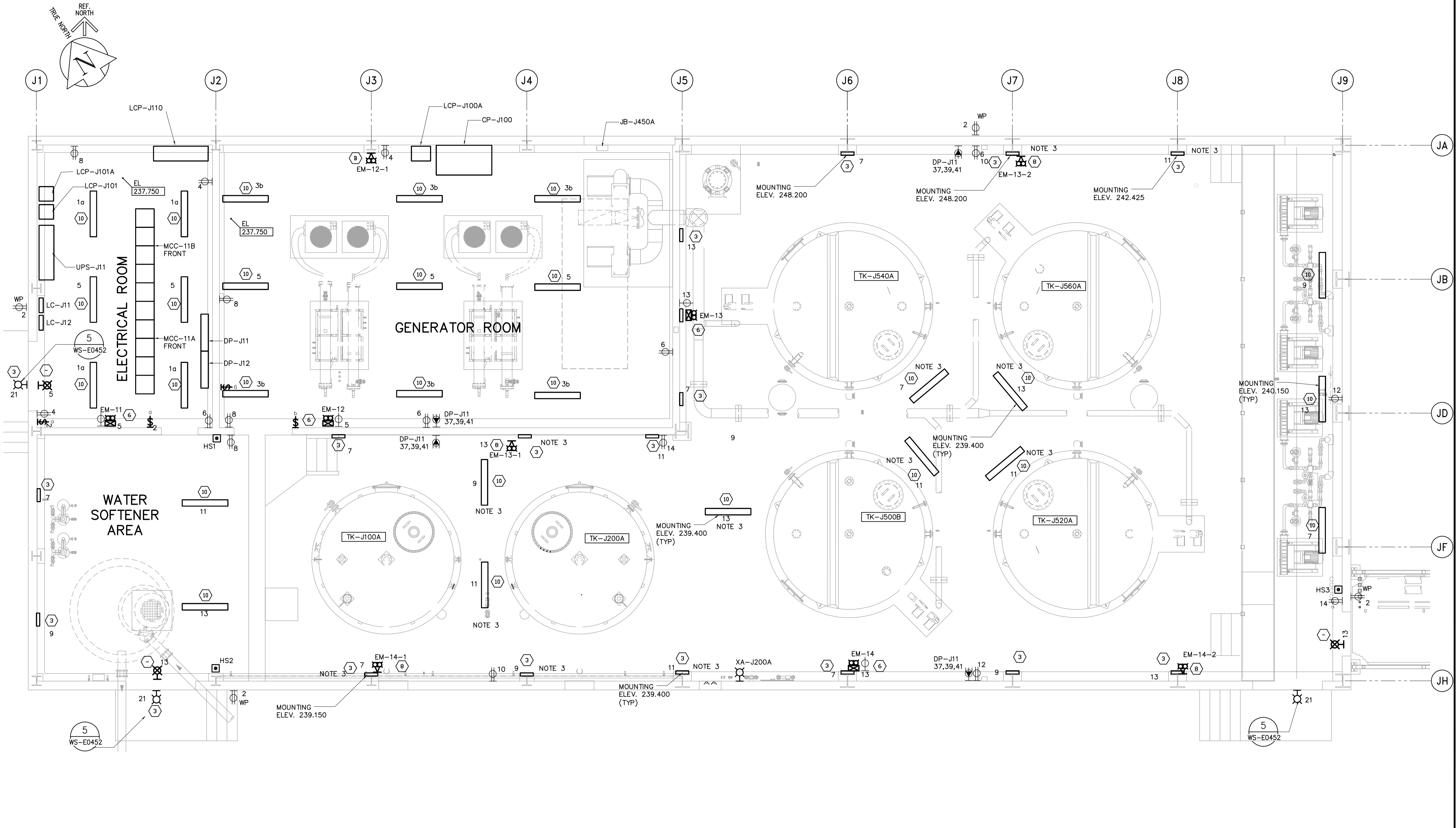
GROUND FLOOR POWER AND LIGHTING PLAN 1:50
