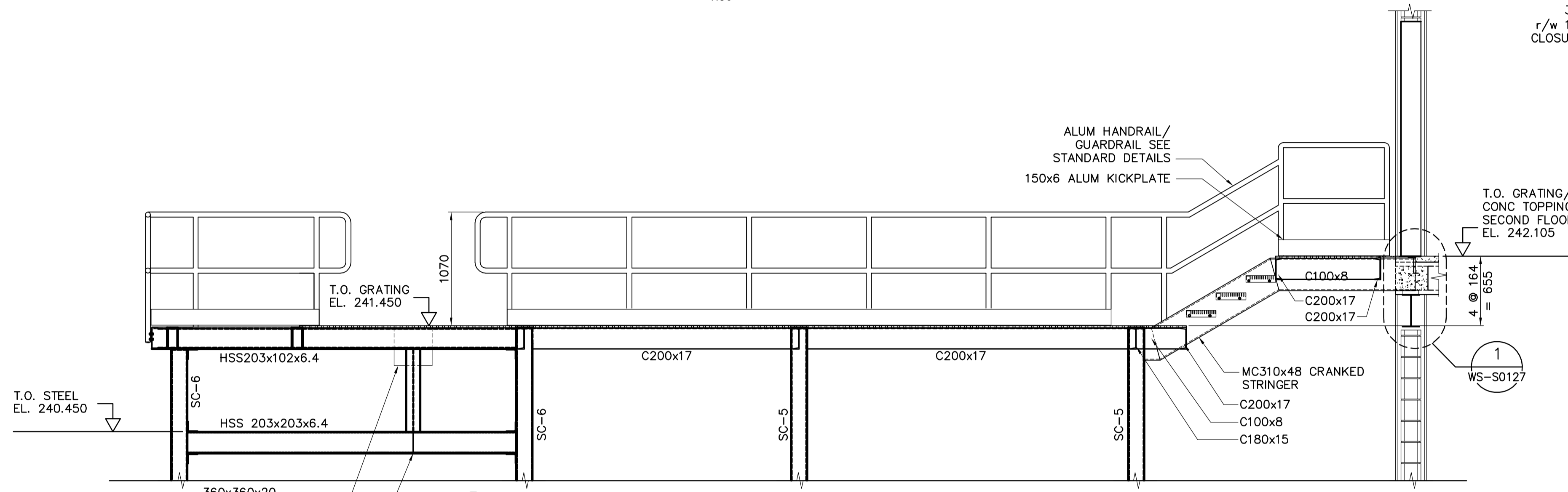
SECTION 3 1:30
