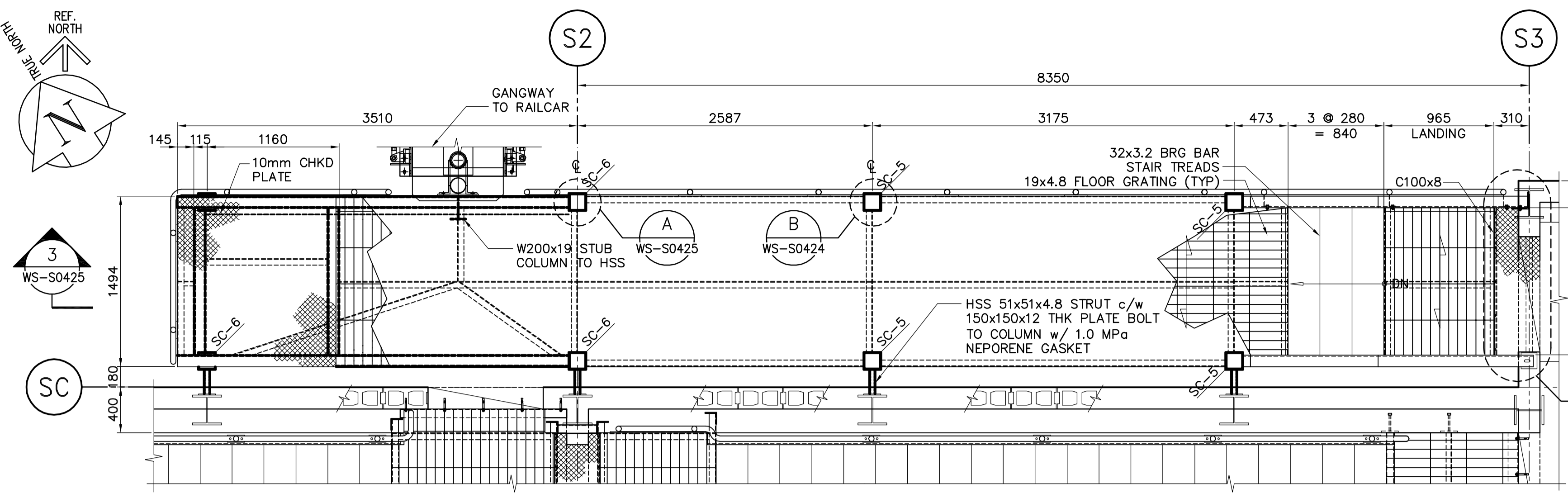
PLAN STAIR # 11 1:30
