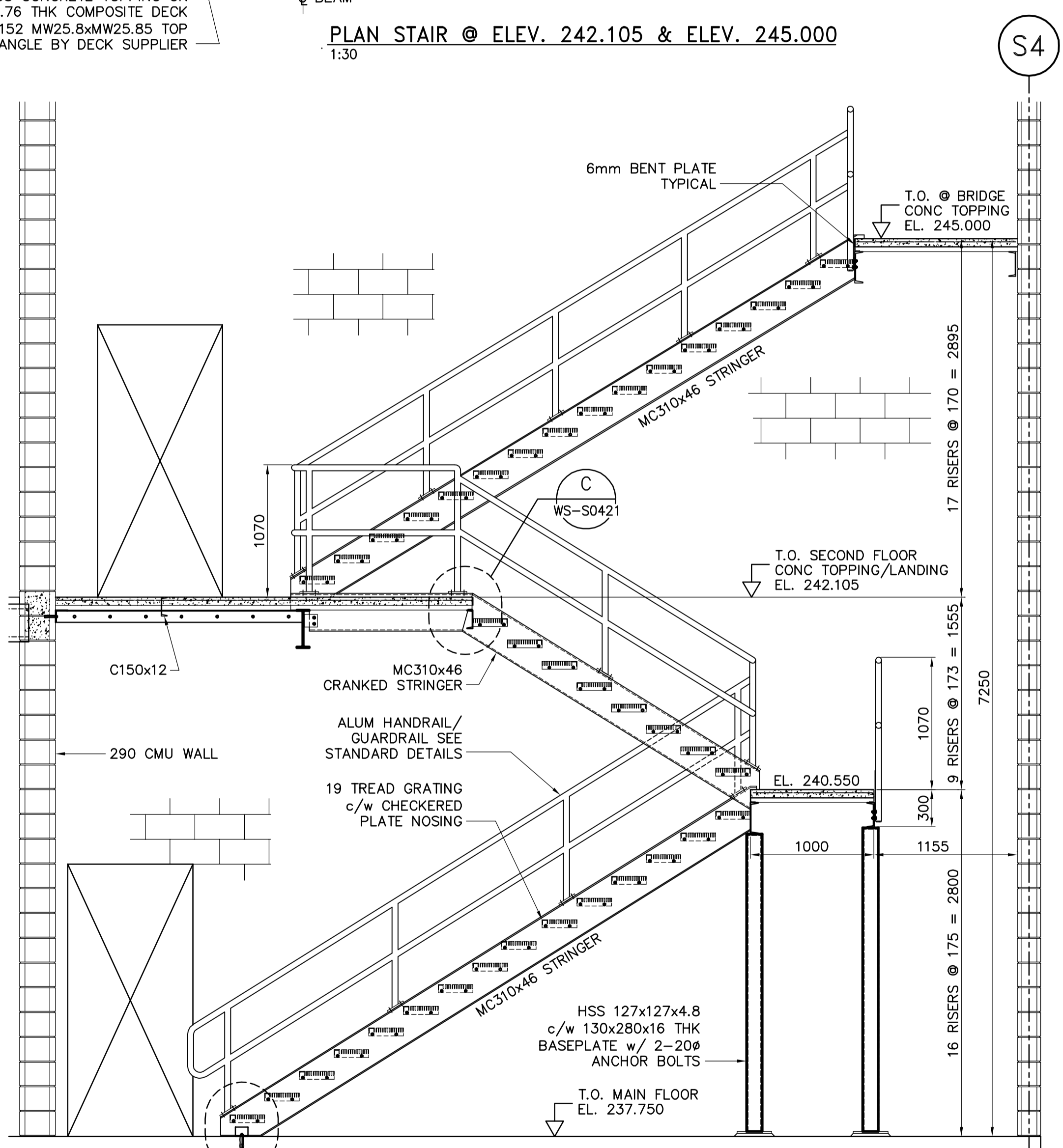
SECTION 4 1:30
