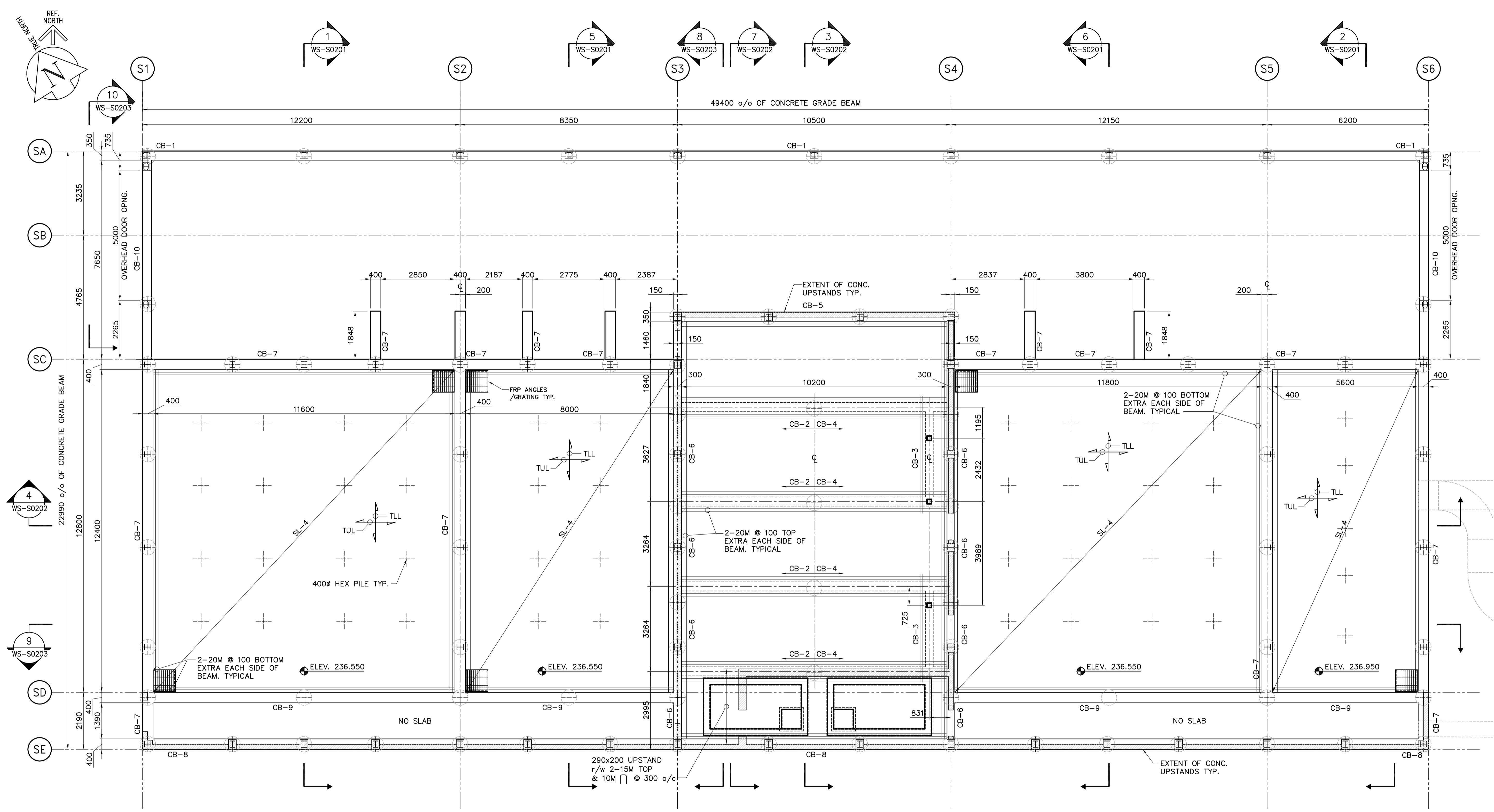
FOUNDATION FRAMING PLAN (LOWER LEVEL) 1:75
