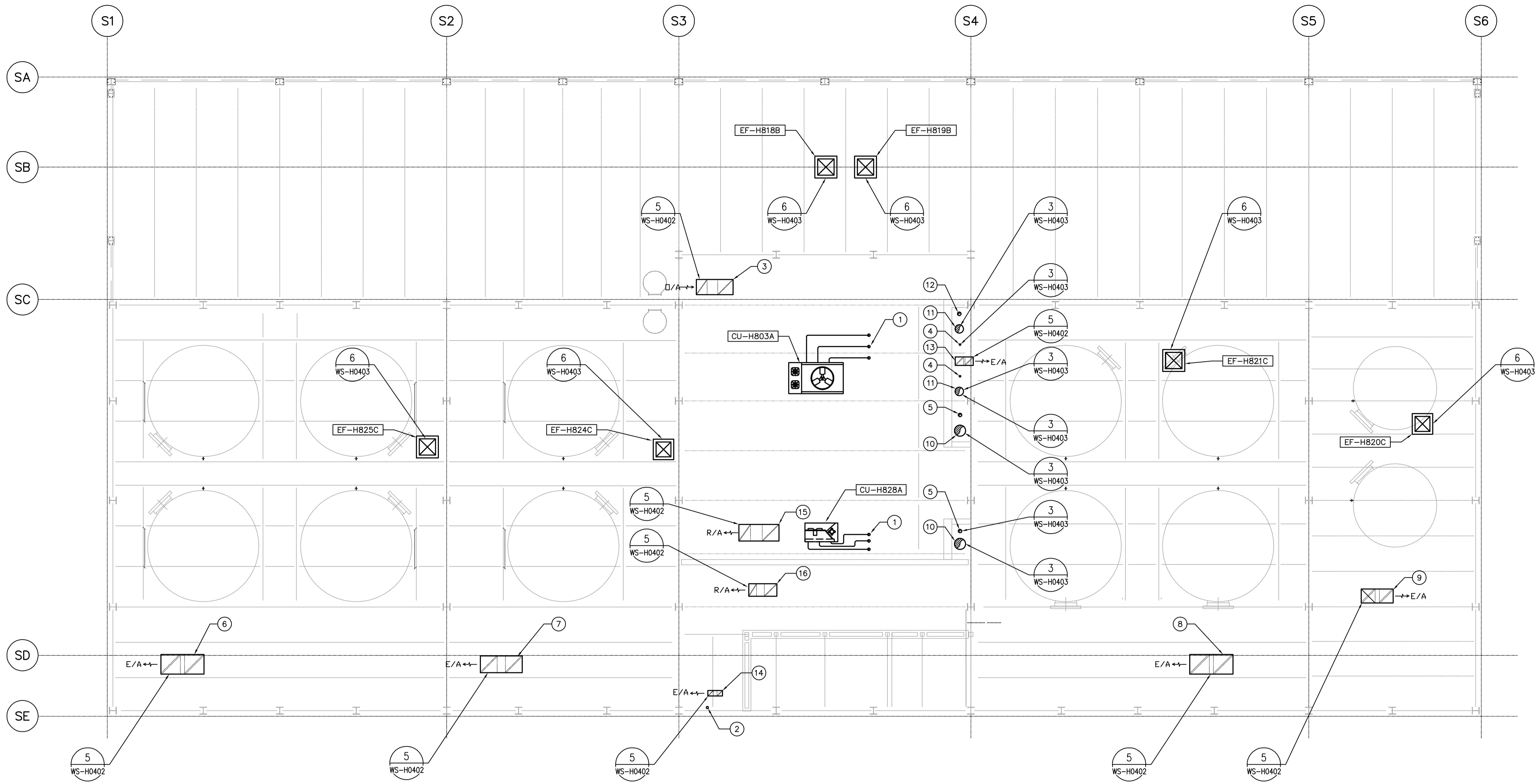
1 ROOF PLAN 1:75
