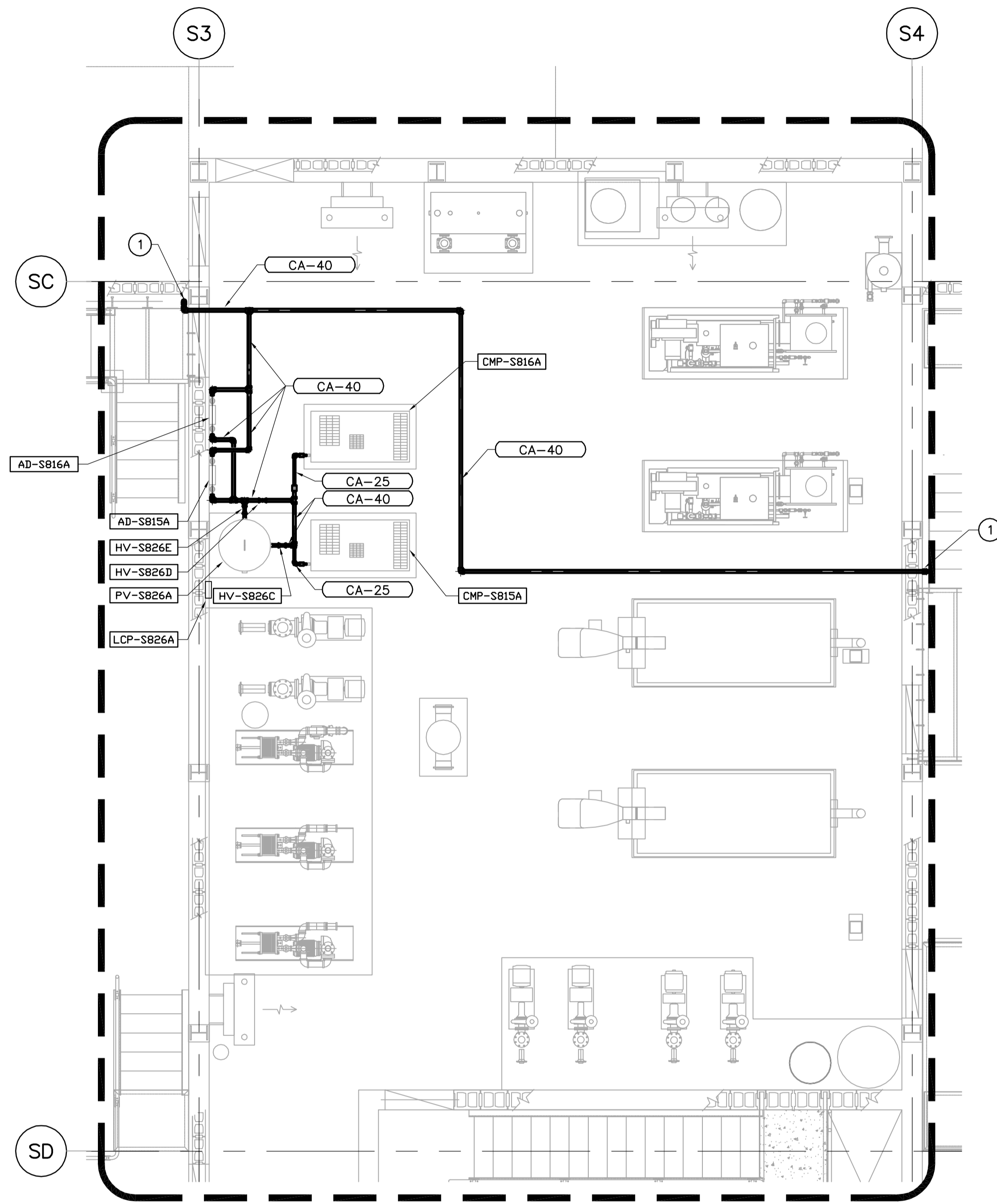
1 - 1:50 MECHANICAL ROOM COMPRESSED AIR PARTIAL PLAN
