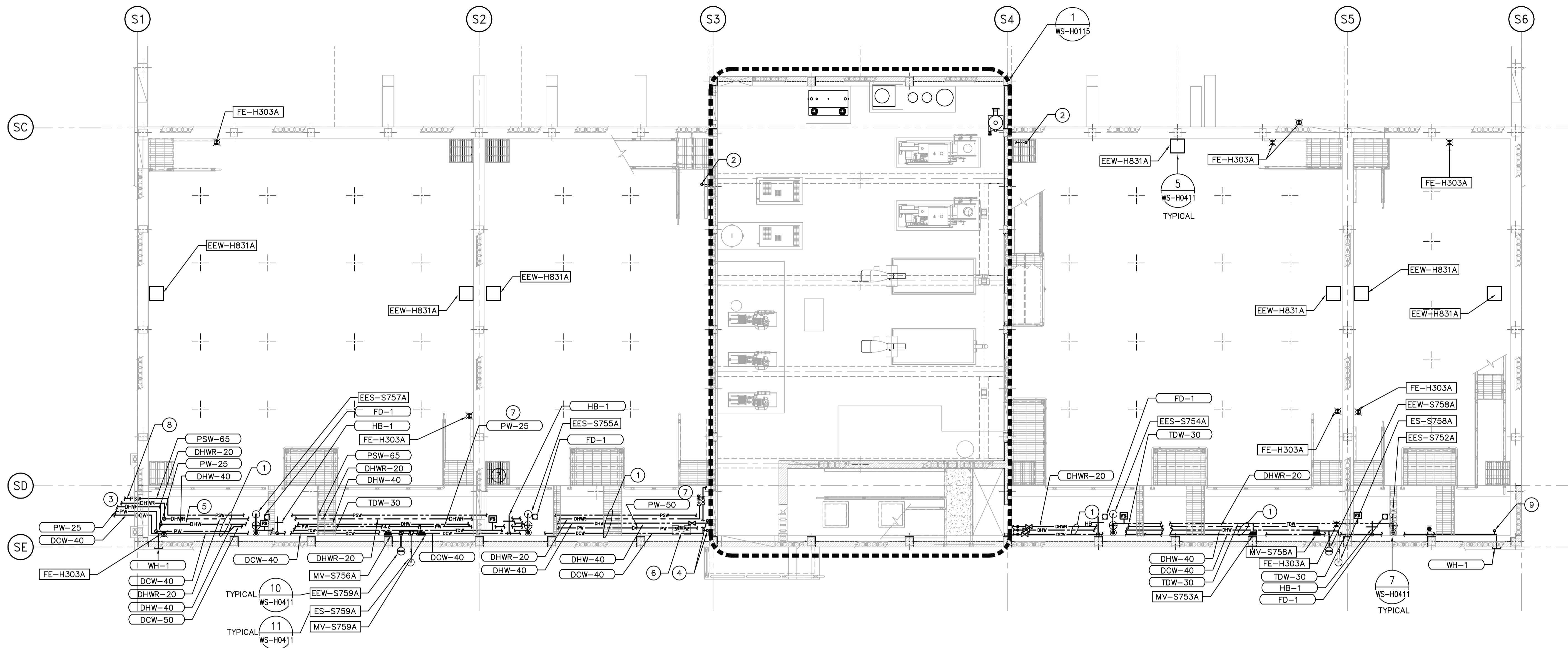
1 MAIN LEVEL PLUMBING PLAN 1:75
