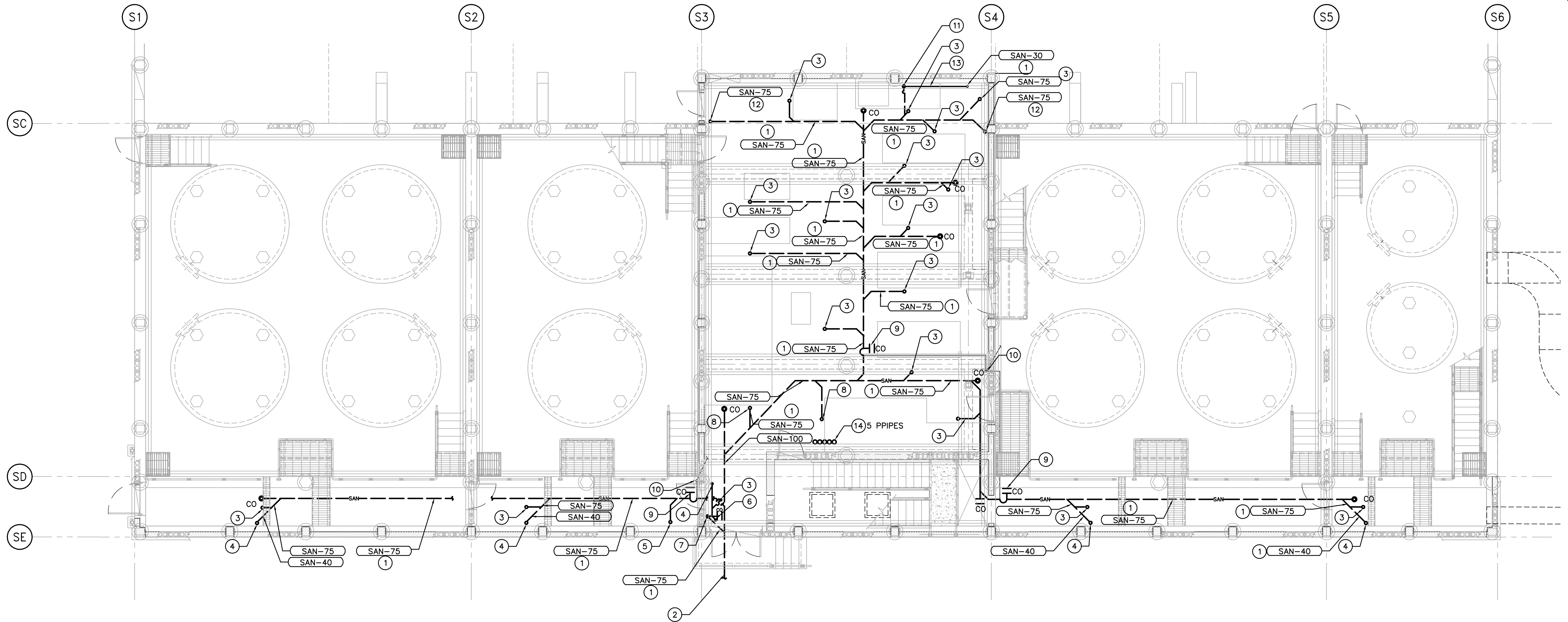
1 FOUNDATION PLUMBING PLAN 1:75
