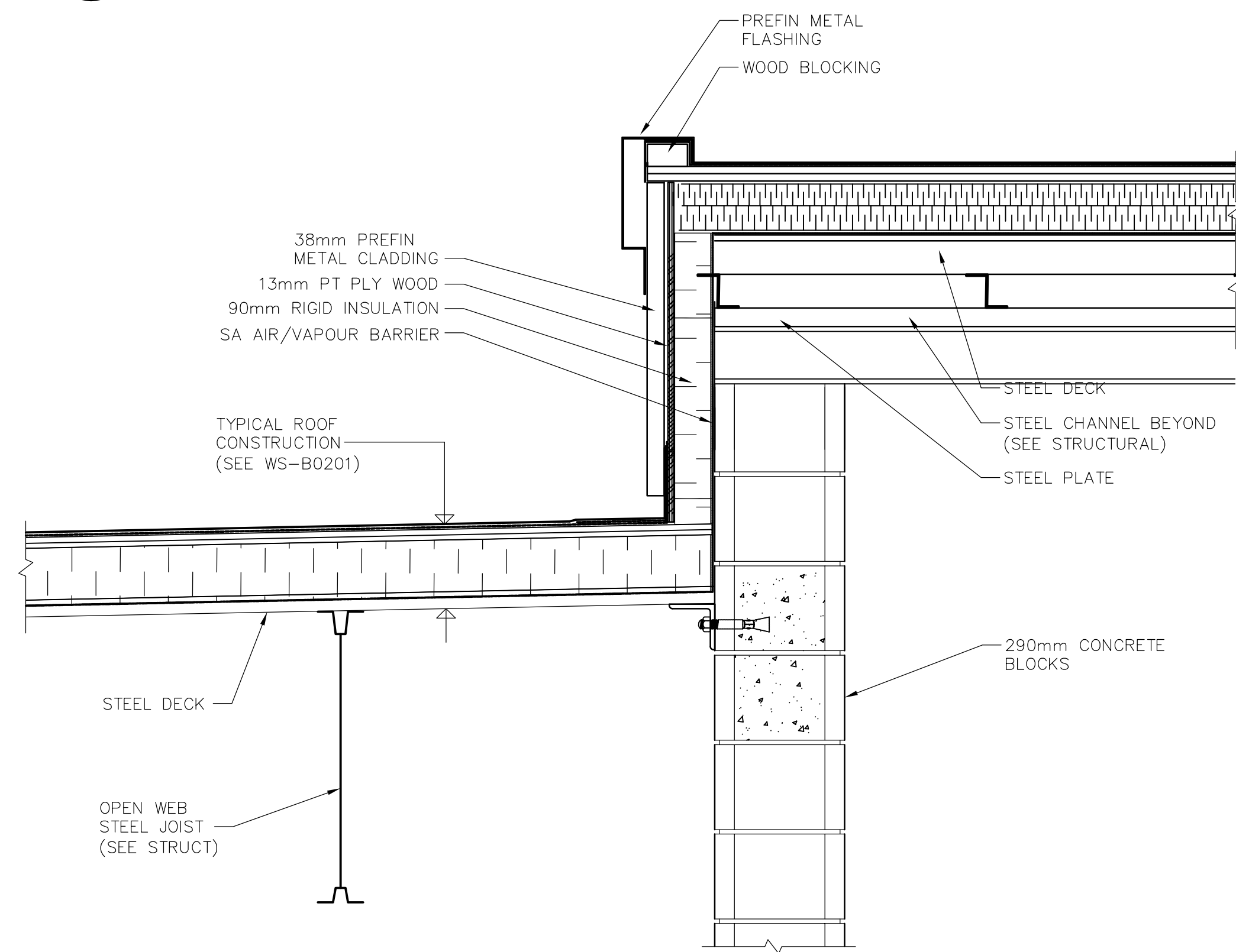
1 DETAIL WS-B0404 1:10
