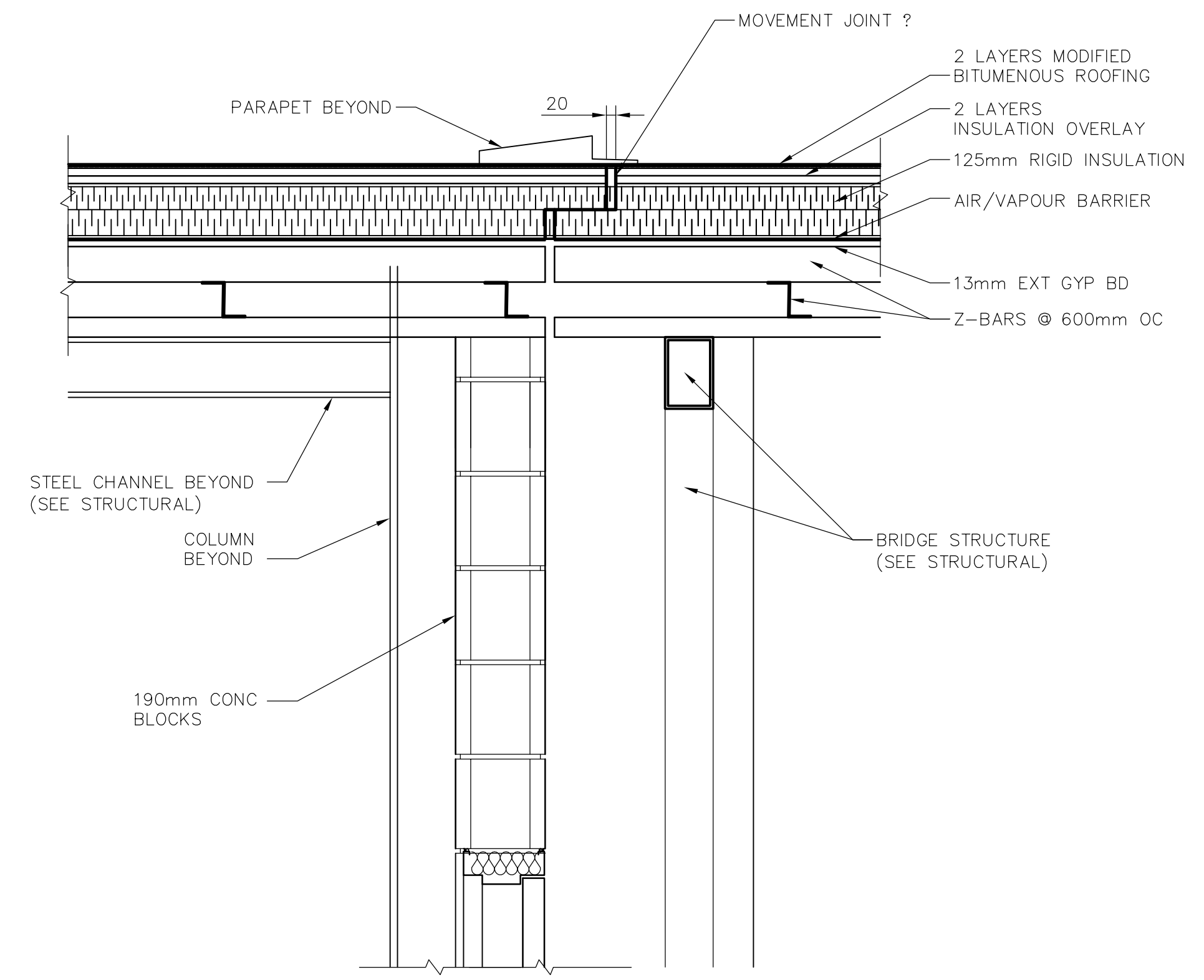
2 DETAIL WS-B0404 1:10
