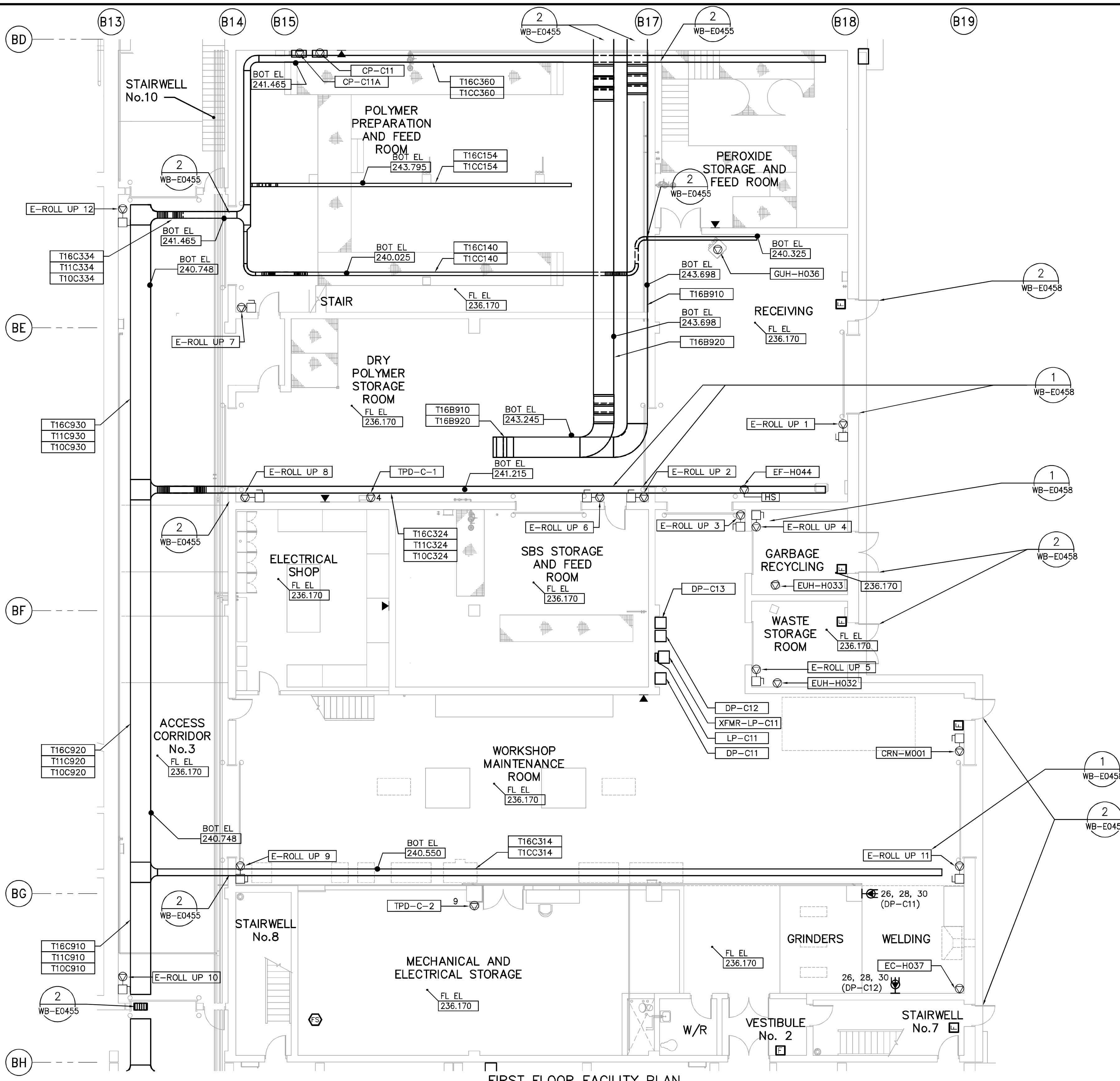
FIRST FLOOR FACILITY PLAN 1:100
