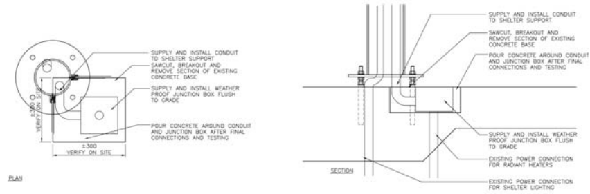
JUNCTION BOX DETAIL FOR ELECTRICAL CONNECTION OF RADIANT HEATERS ON EXISTING SHELTER BASES
