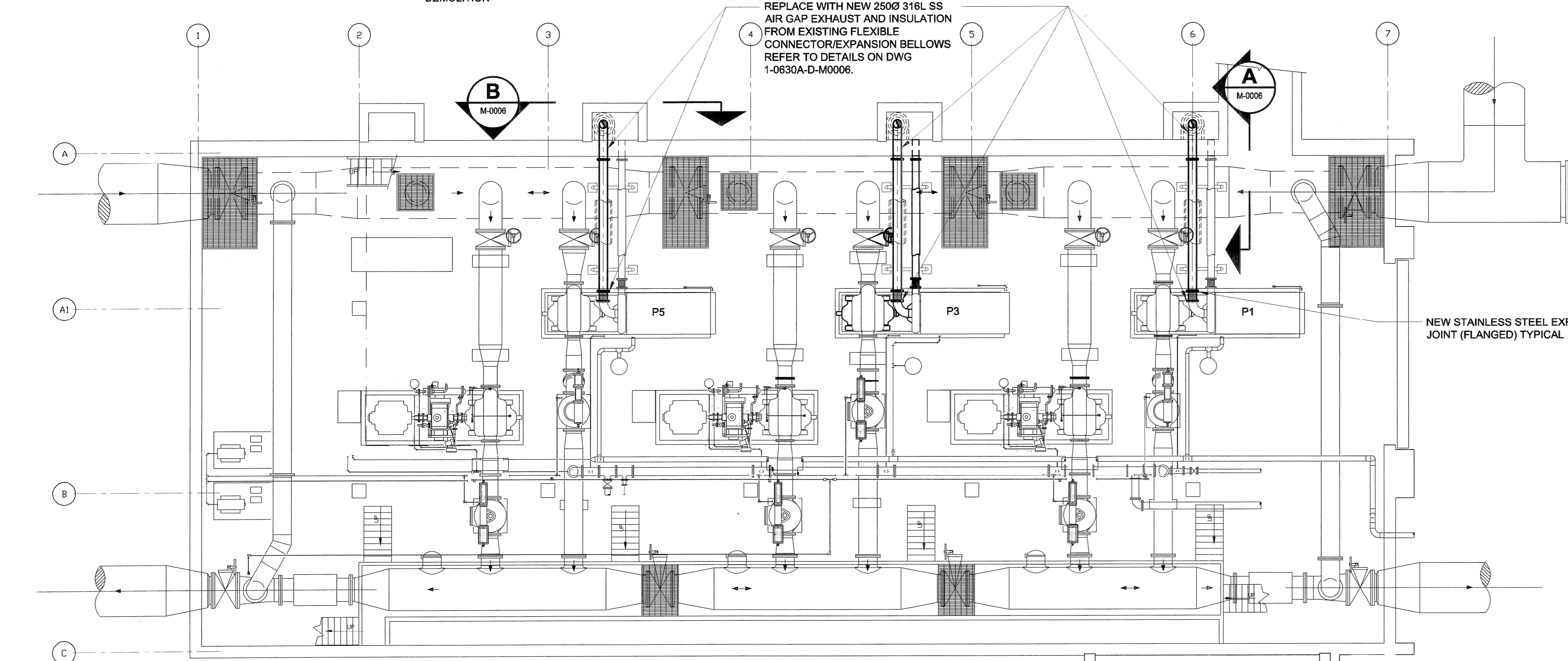
PLAN 2 SCALE 1:100 NEW CONSTRUCTION
